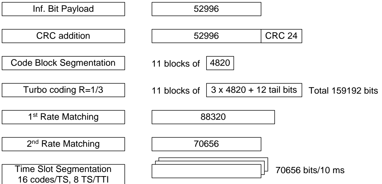
Figure A.11: Coding for HS-PDSCH fixed reference channel with 16-QAM modulation for the PA3 PB3, and VA30 Channels - Category 8
