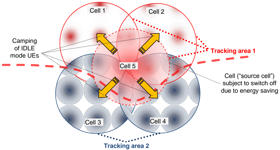
Figure 5.1.5-1: Capacity enhancing cell being switched off (overlaid intra-RAT case)
