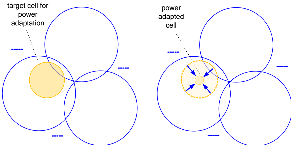
Figure 5.5.1-1: Power adaption for capacity enhancing cells in 3GPP macro network, due to energy saving (left: normal mode, right: energy saving mode)
