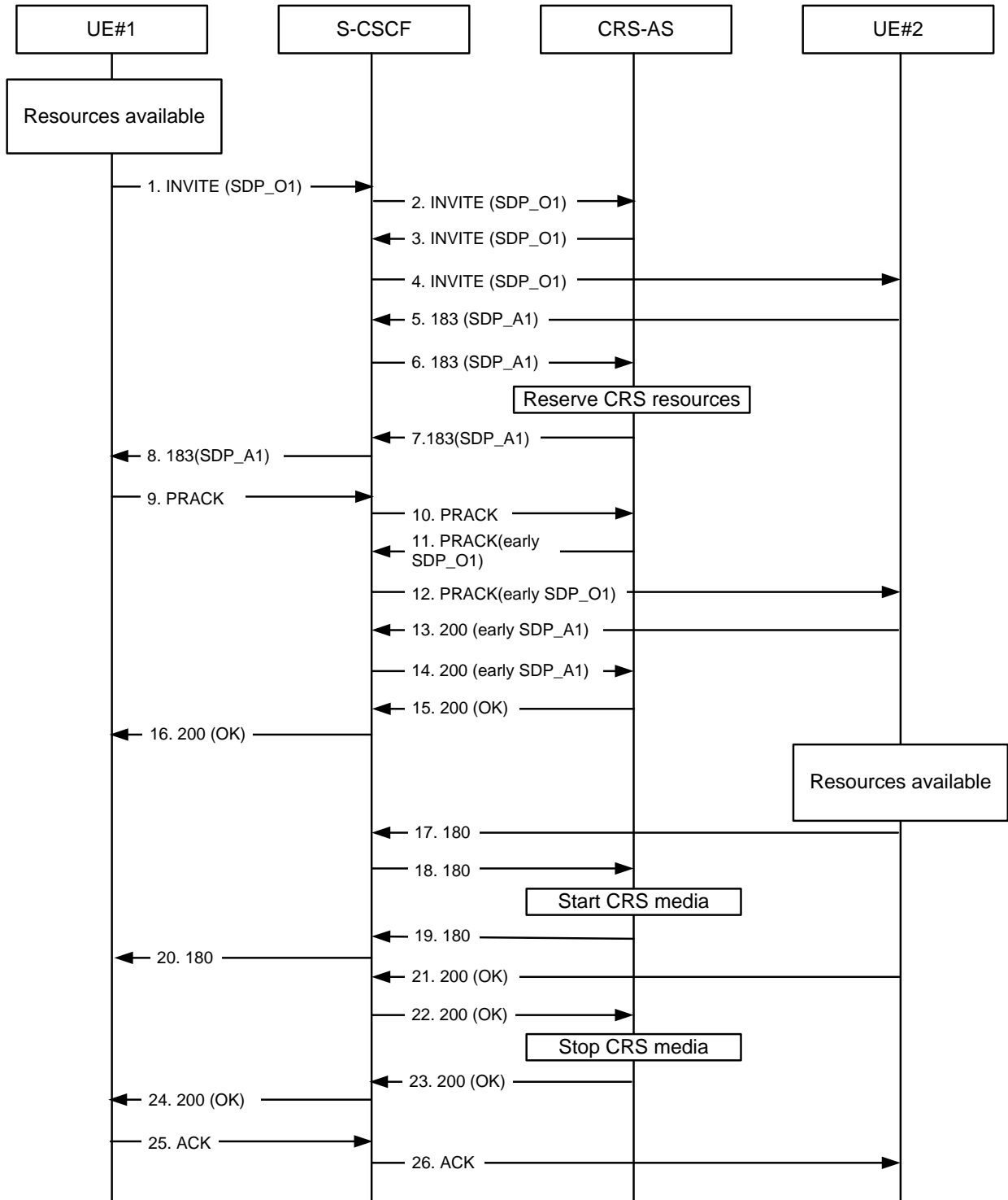
Figure A.2.4-1: CRS, UE#2 does not have resource available
