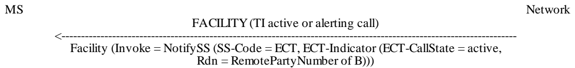
Figure 5: Notification of invocation to previous-active or previous-alerting remote party
