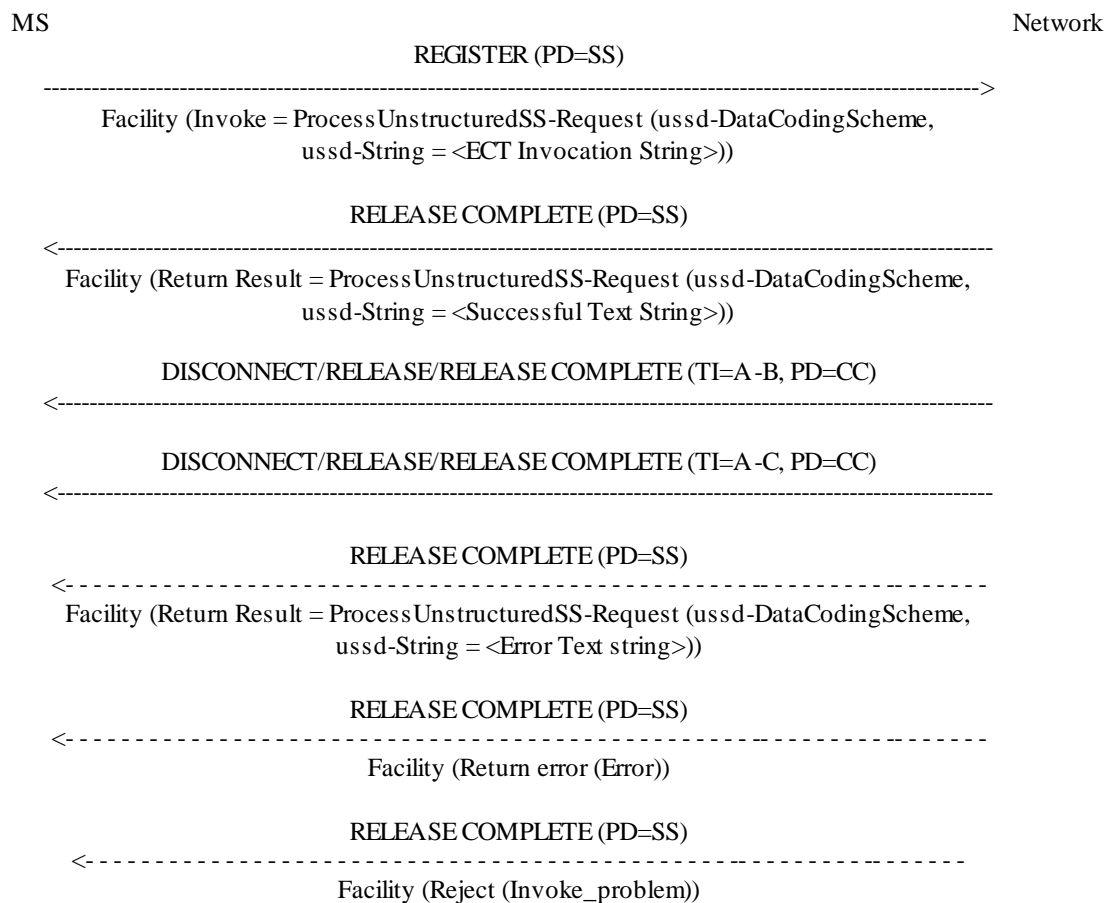
Figure 6: Invocation of Explicit Call Transfer for non supporting MSs
