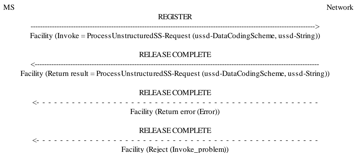
Figure 6.1: Mobile initiated USSD operation, network does not request further information
