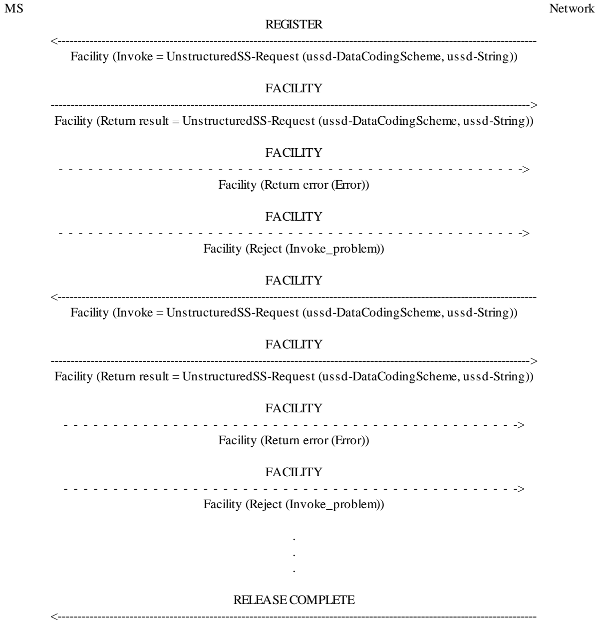
Figure 5.2: Multiple network initiated USSD request
