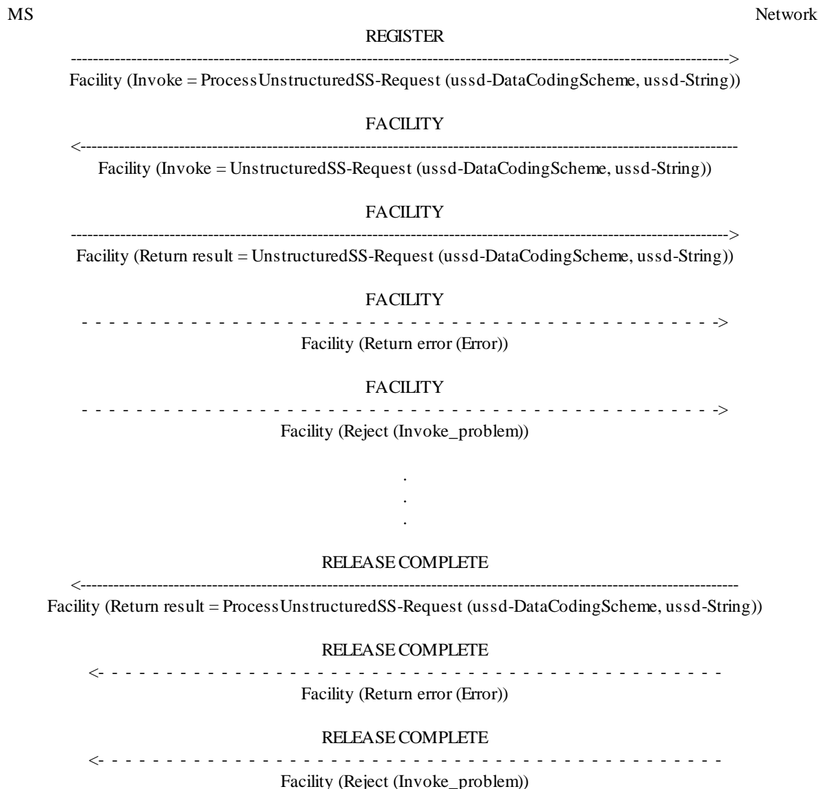
Figure 6.2: Mobile initiated USSD operation, network requests further information
