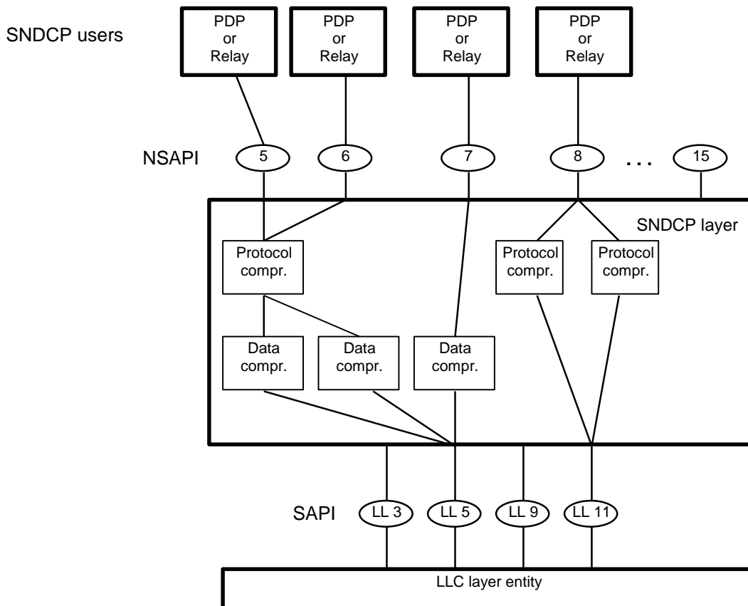
Figure 8: An example for the usage of NSAPIs, SNDSCP functions, and SAPIs
