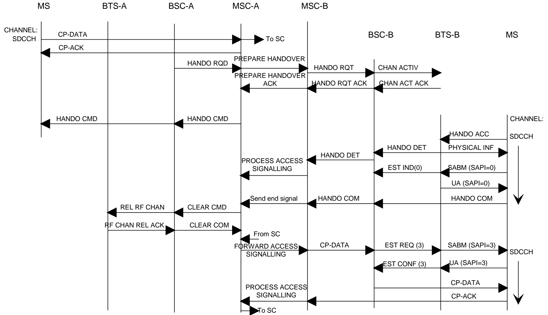
Figure F6/3GPP TS 24.011: Inter/MS network handover during Short Message transfer on SDCCH
