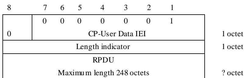
Figure 8.2/3GPP TS 24.011: CP-User data element layout
