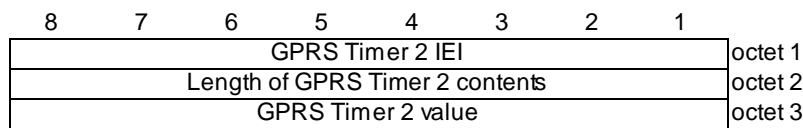
Figure 10.5.147/3GPP TS 24.008: GPRS Timer 2 information element
