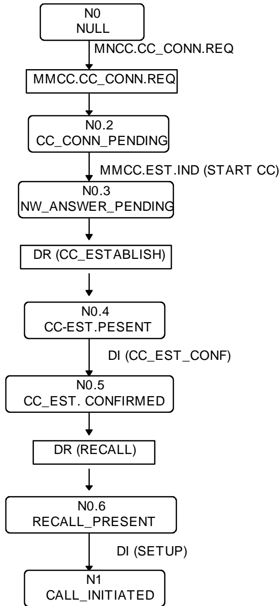
Figure 5.1b.1/3GPP TS 24.008 Overview call control protocol/Network side, extension
