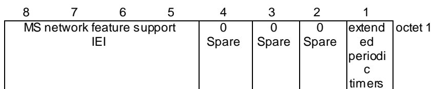
Figure 10.5.1.15/3GPP TS 24.008: MS network feature support information element
