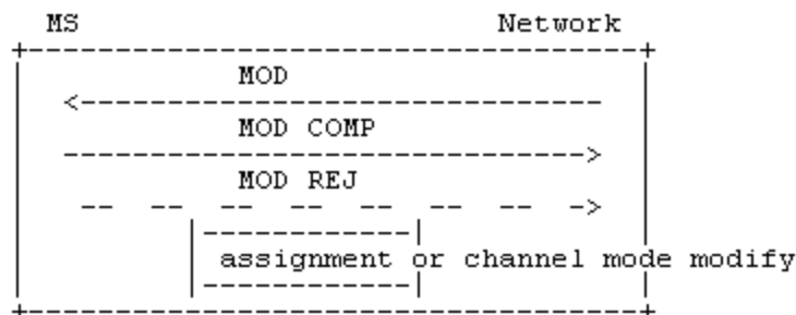
Figure 5.10b/3GPP TS 24.008 In-call modification sequence initiated by network
