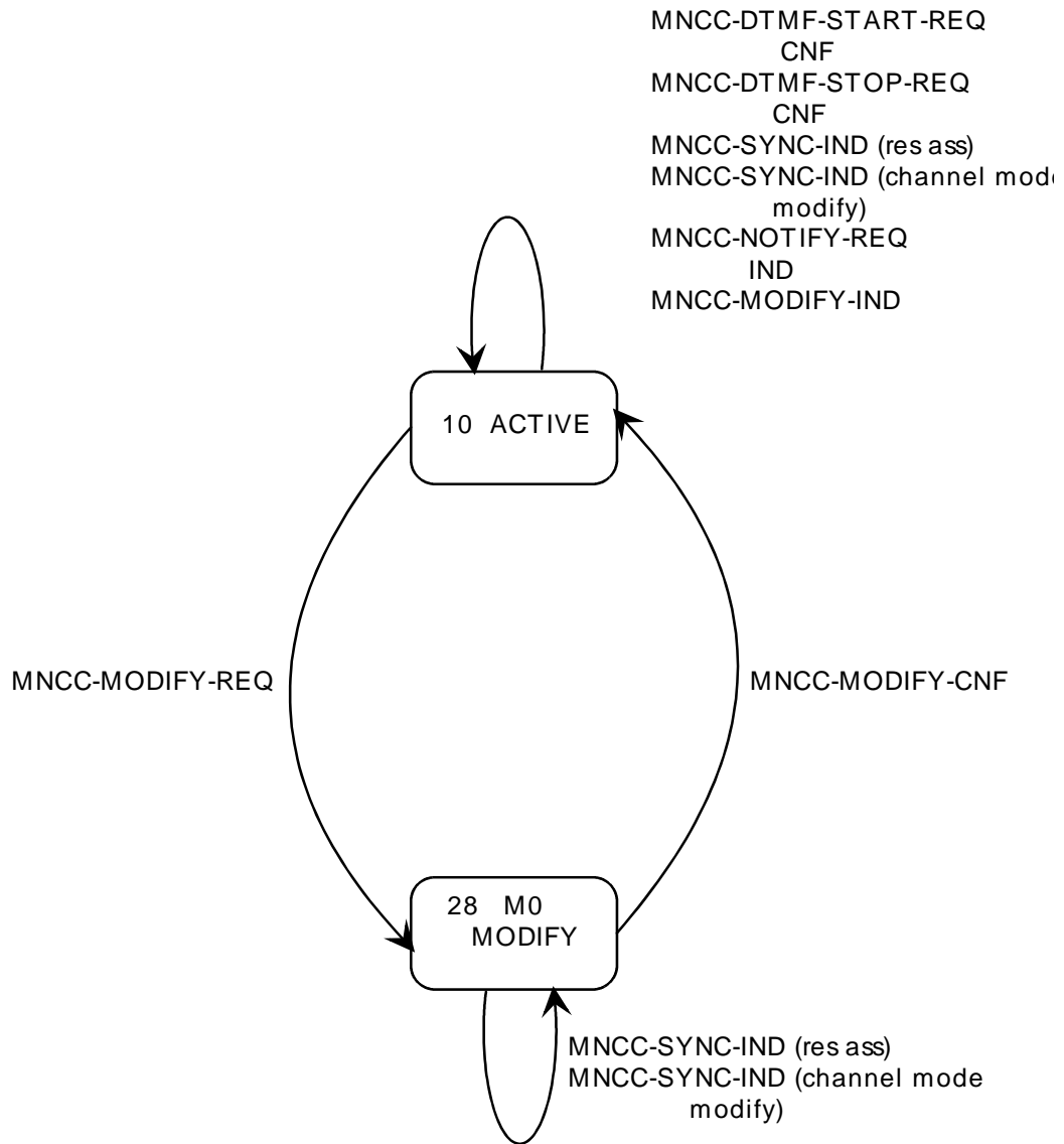
Figure 6.2: Service graph of Call Control entity - MS side Active state (page 2 of 2)
