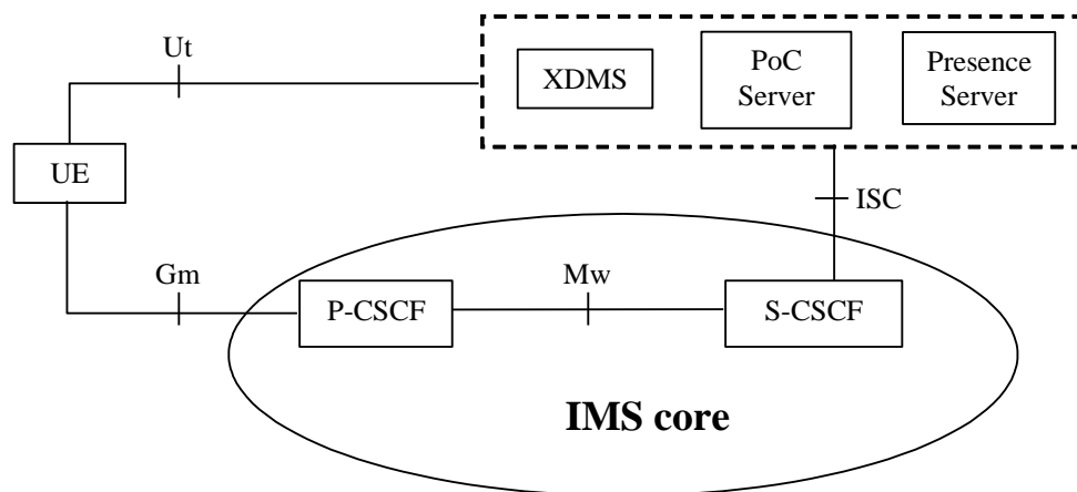
Figure 5-1: PoC service elements in the IMS architecture
