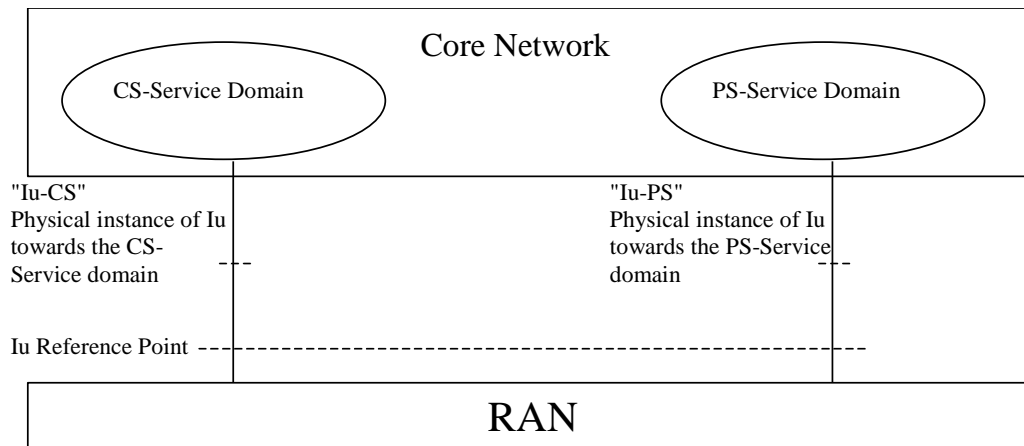
Figure 1: Iu Reference point, and the Iu-CS and Iu-PS physical instances
