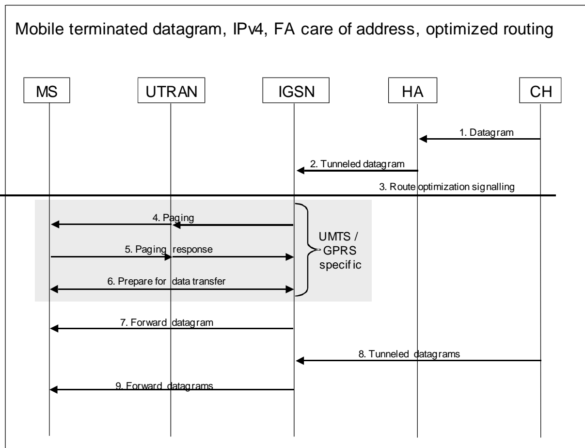
Figure 11.7.2b: Delivery of mobile terminated datagrams, optimised routing
