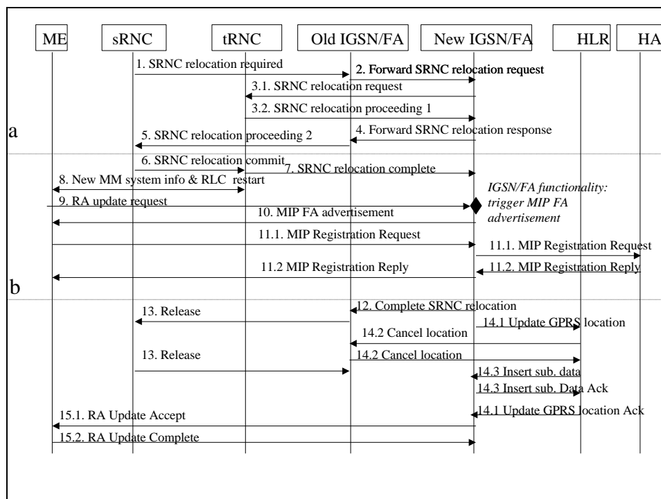
Figure 11.6a: SRNS relocation in a step 3 network
