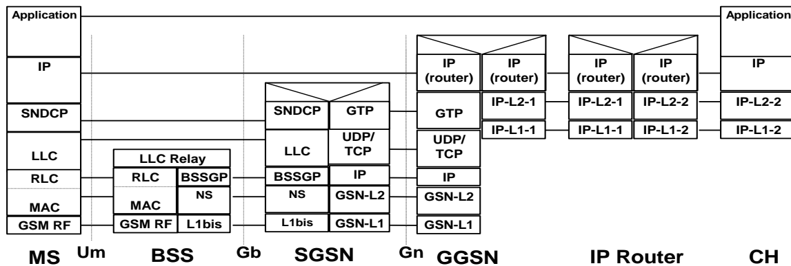
Figure 8.6a: Protocol stack for GPRS including the Internet
