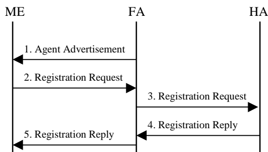
Figure 8.6b: Packet routing in a Mobile IP network in Registration
