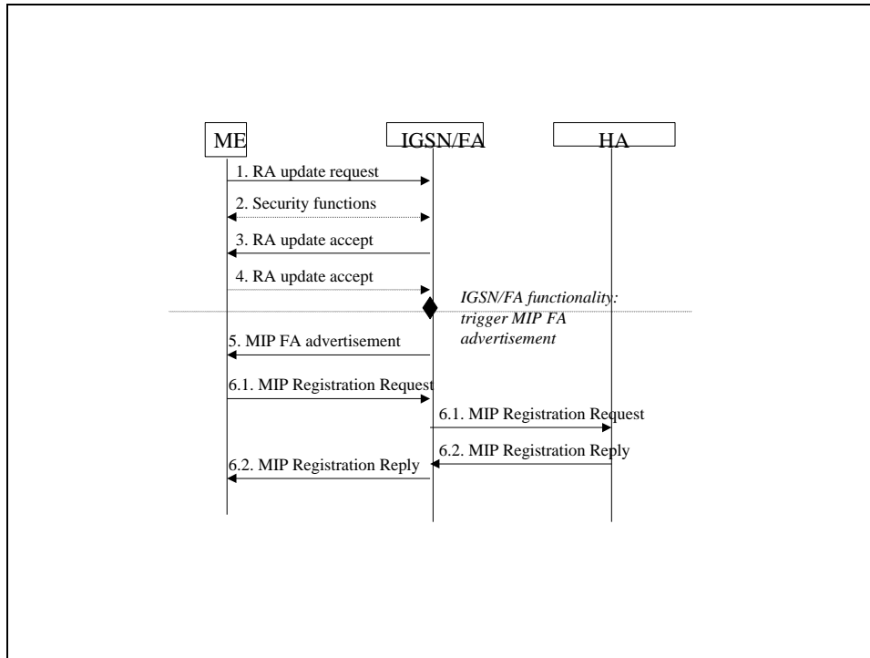
Figure 11.5.2a: Intra IGSN Routing Area Update
