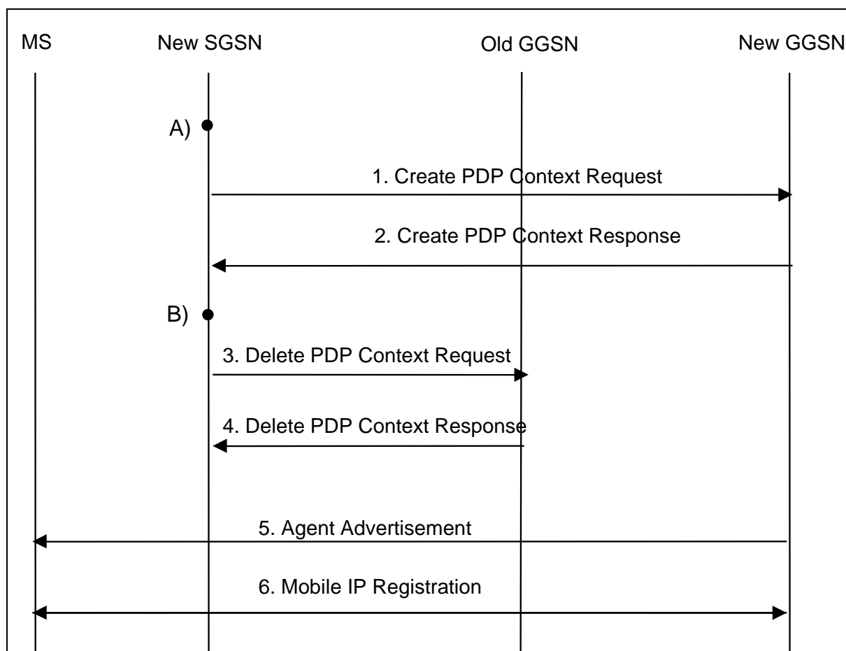
Figure 10.1a: The GGSN/FA handover
