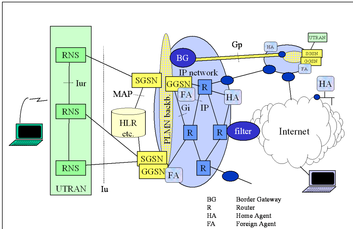
Figure 7.2a Core network architecture where GPRS MM handles active mobiles and Mobile IP(+) streamlining at inter SGSN handover. The SGSN and GGSN are here co-located
