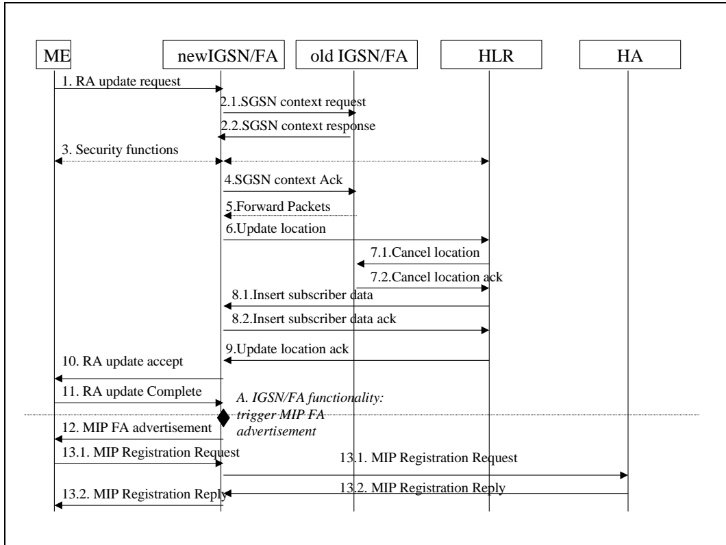
Figure 11.5.1a: Inter IGSN RA update
