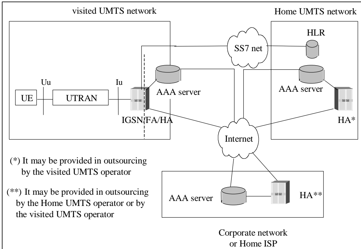
Figure 8.7.1b: UE not attached to the Home UMTS operator
