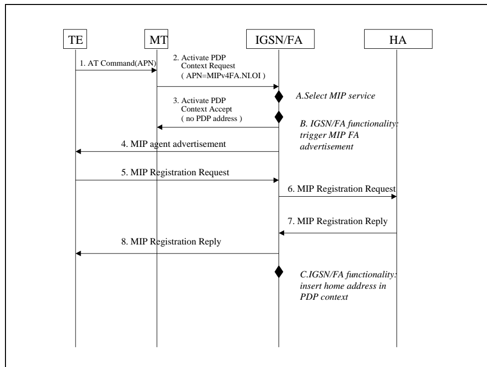
Figure 11.4a: Session activation in a step 3 network
