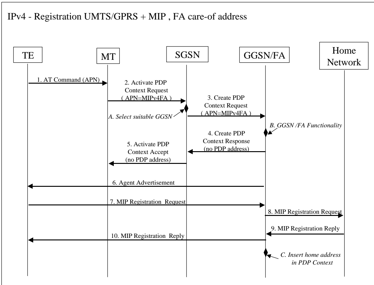
Figure 9.4a, PDP Context activation with Mobile IP(+) registration (the PPP setup and UMTS/GPRS attach procedure not included)
