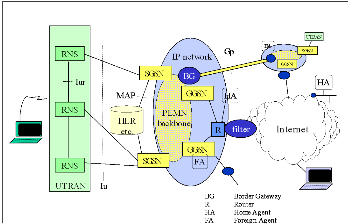
Figure 7.1a: Core network architecture with GPRS MM in and between GPRS PLMNs and Mobile IP MM between different types of systems and optionally between GPRS PLMNs
