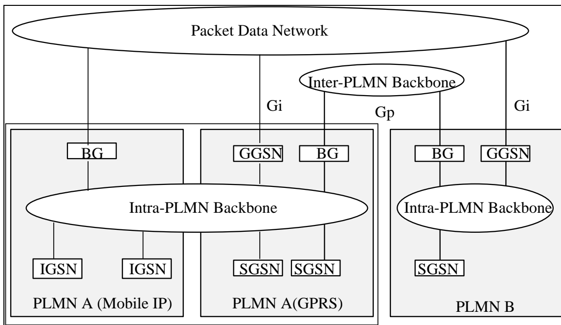
Figure 12.2.2a: Interoperability with GPRS
