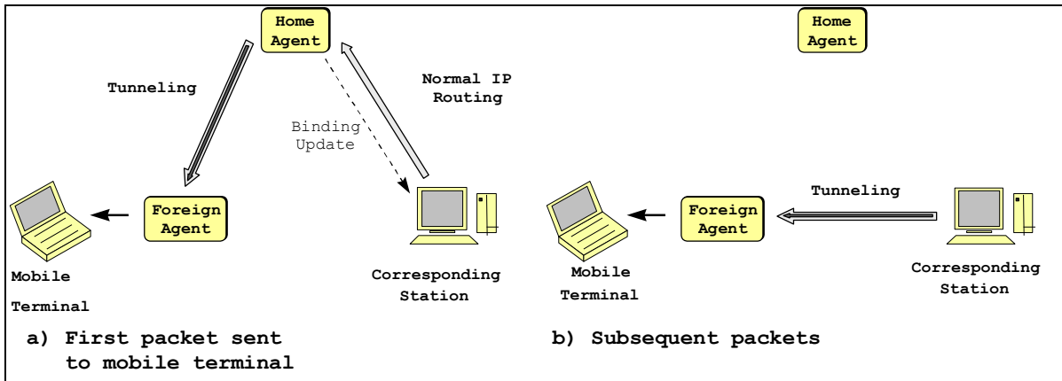
Figure A.2: Route Optimisation in IPv4
