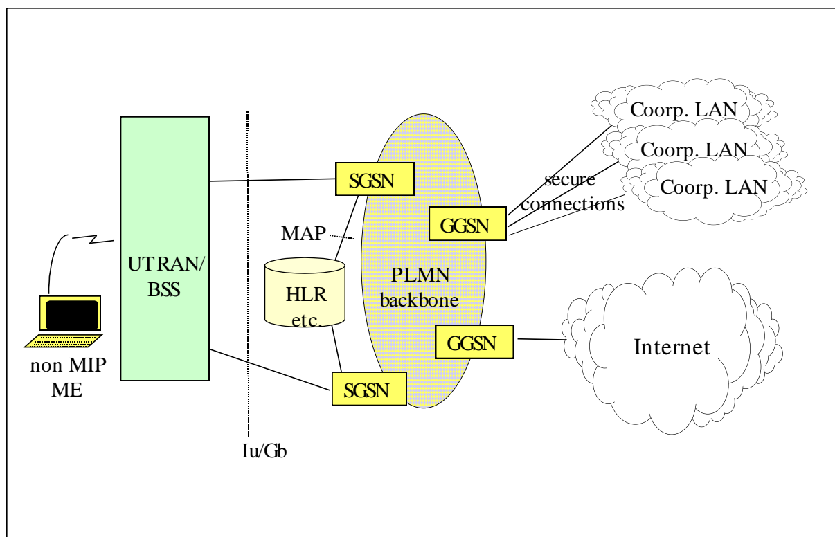
Figure 12.2.1.1a: The situation when the PLMN backbone mobility is handled with GTP. The mobile stays with the same GGSN throughout the UMTS/GPRS session
