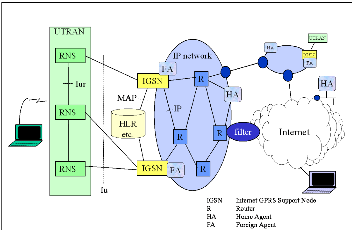
Figure 11a: Step 3 network architecture
