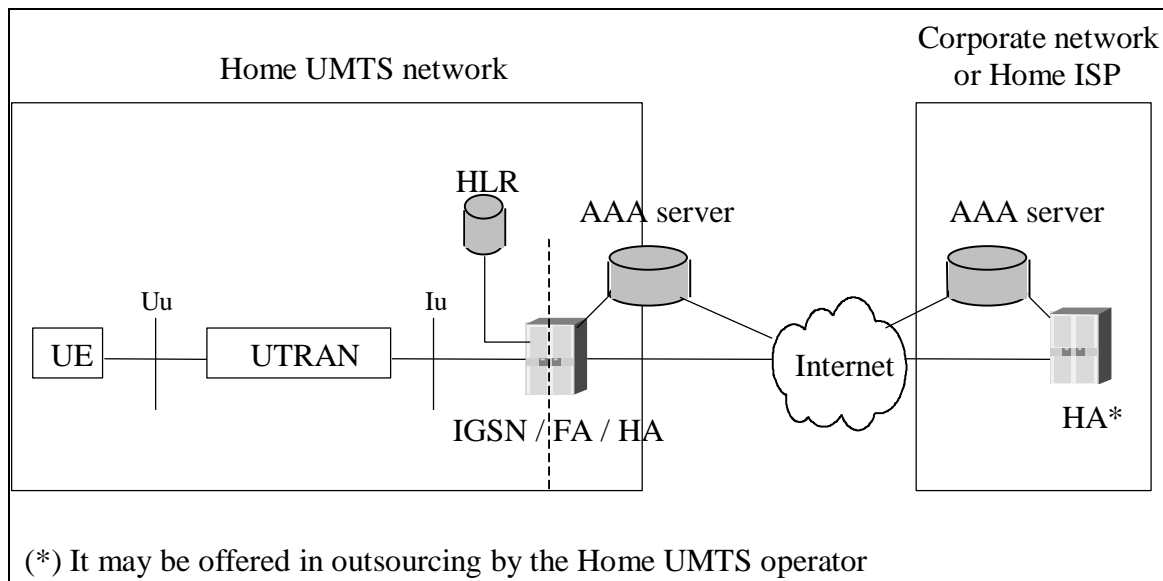
Figure 8.7.1a: UE attached to the Home UMTS operator
