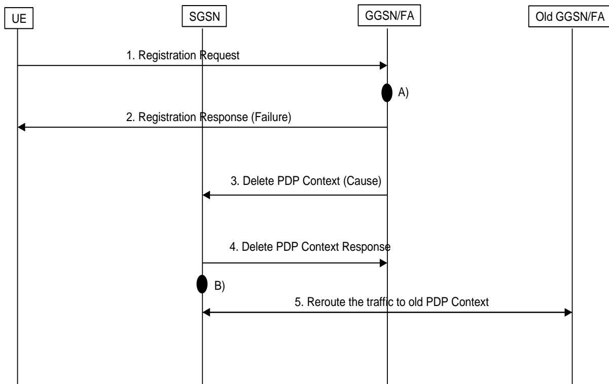
Figure 10.2a: Mobile IP registration failure
