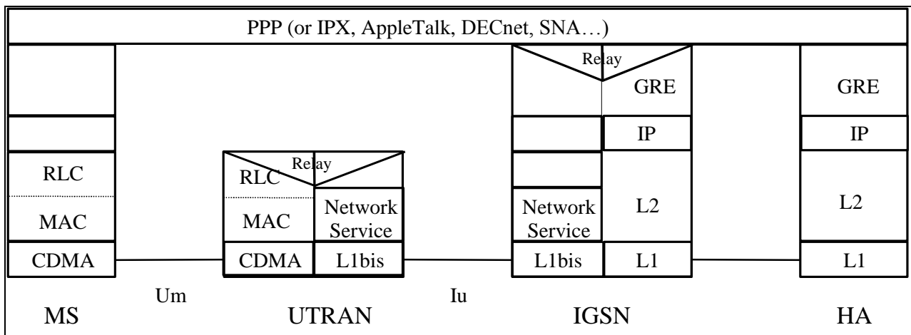
Figure 11.8.2a: Multiprotocol support in Mobile IP(+)
