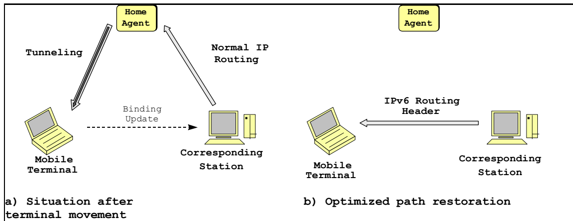
Figure A.5: Route Optimisation in IPv6
