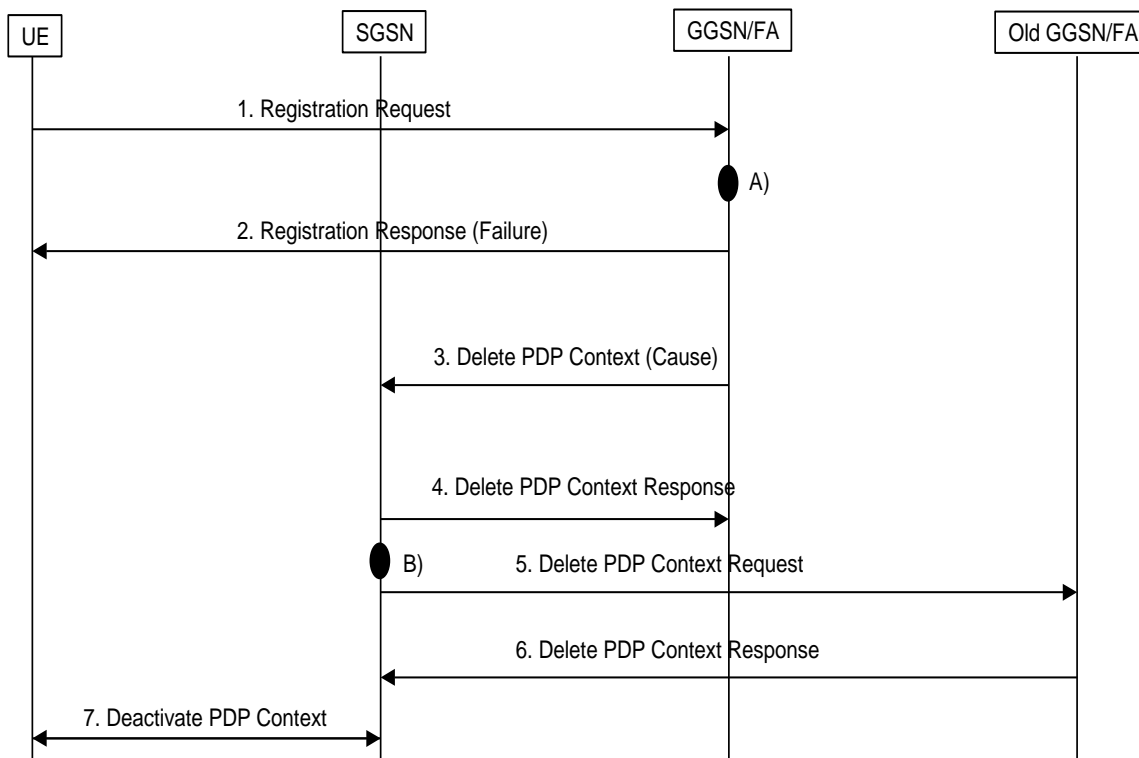
Figure 10.2b: Case when no fall-back is possible
