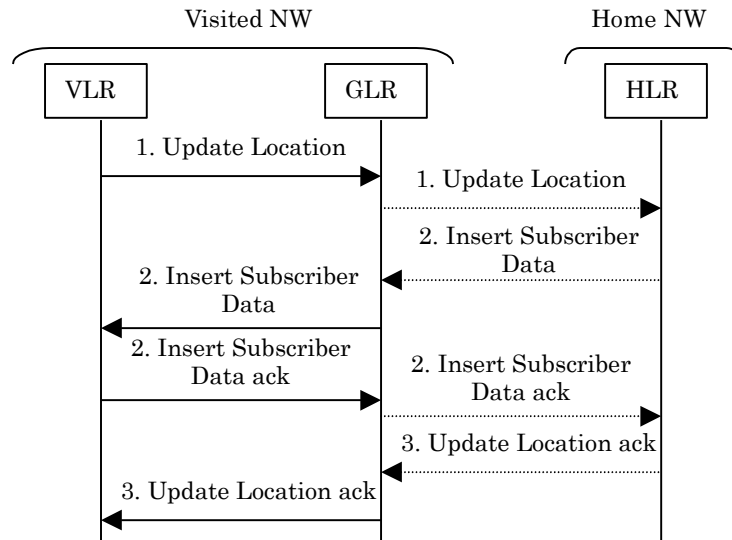
Figure 14: Location Updating Screening
