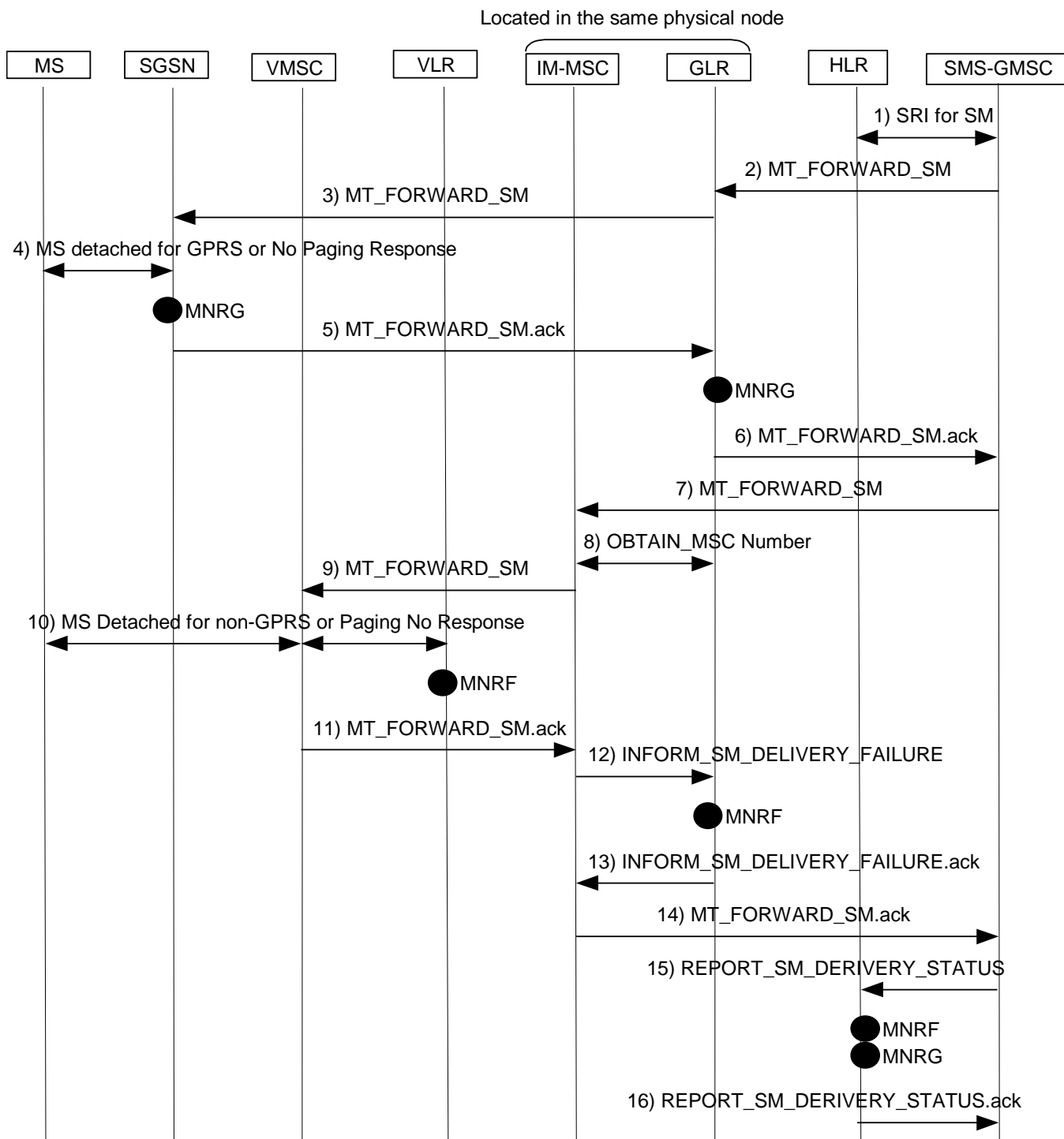
Figure 32: unsuccessful SMS MT over MSC and SGSN
