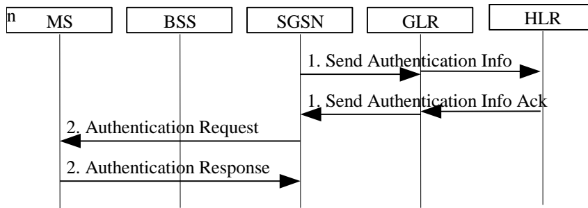
Figure 17: Authentication Procedure
