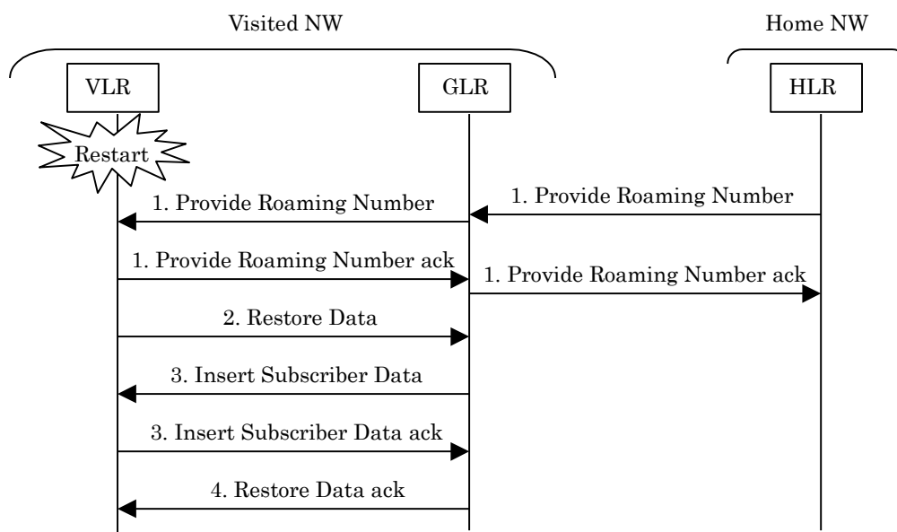
Figure 26: Restoration of the VLR by Mobile Terminated call
