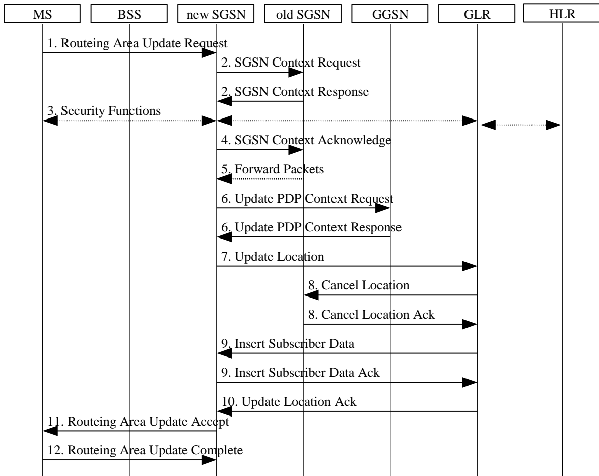
Figure 18: Inter SGSN Routing Area Update Procedure
