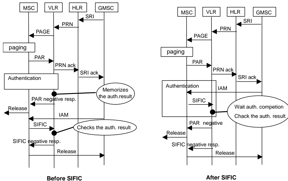
Figure 3 Authentication Failure
