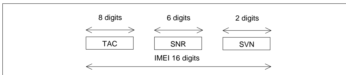
Figure 3: Structure of IMEISV
