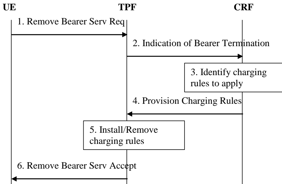
Figure 6.3: Bearer Service Termination
