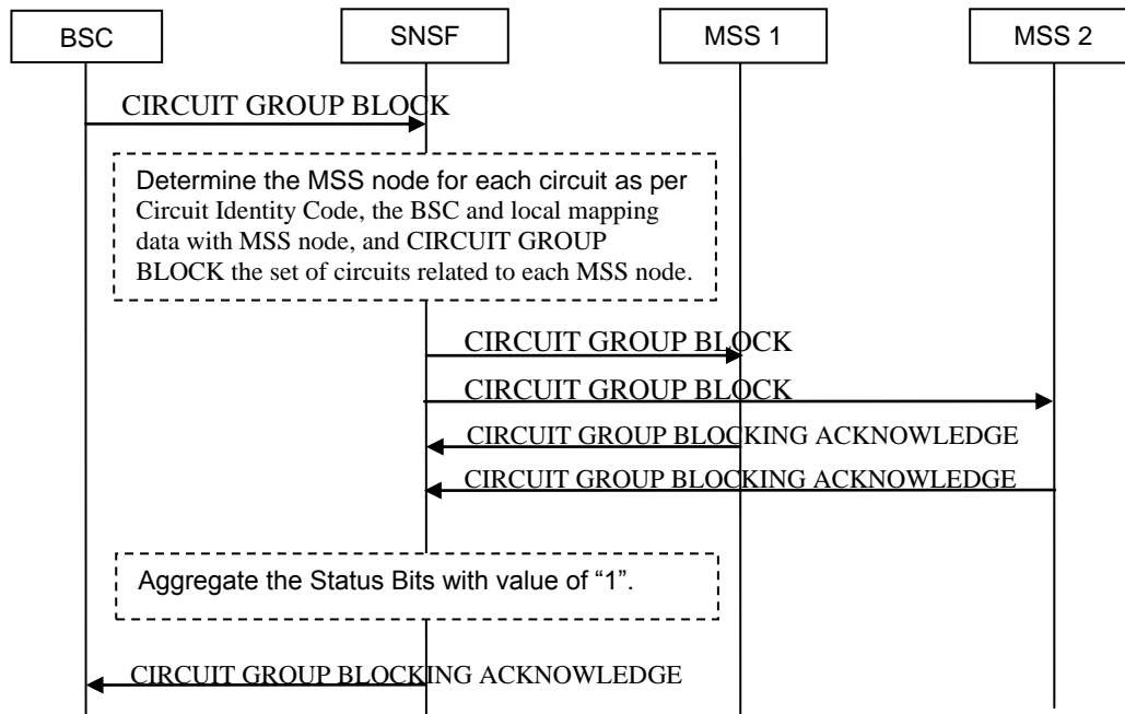
Figure 5.6.3.2.10.1: Uplink TDM Circuit Management Message Handling at the SNSF (SNSF distributes the messages as per circuit identity)
