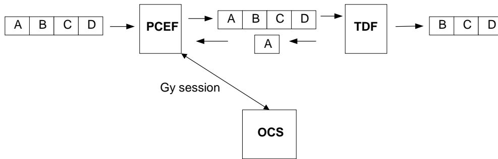
Figure 6.3.7.3.2-1 SDF-based charging for uplink traffic
