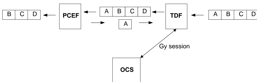
Figure 6.3.7.3.1-1 Application-based charging for downlink traffic
