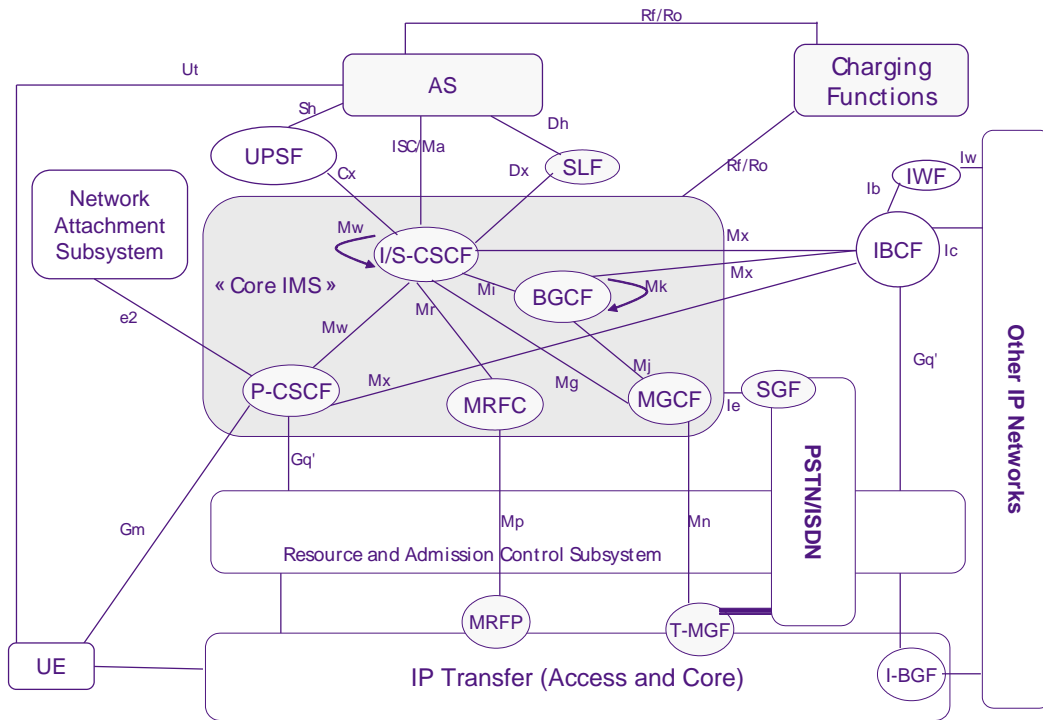
Figure 3: NGN IMS overview
