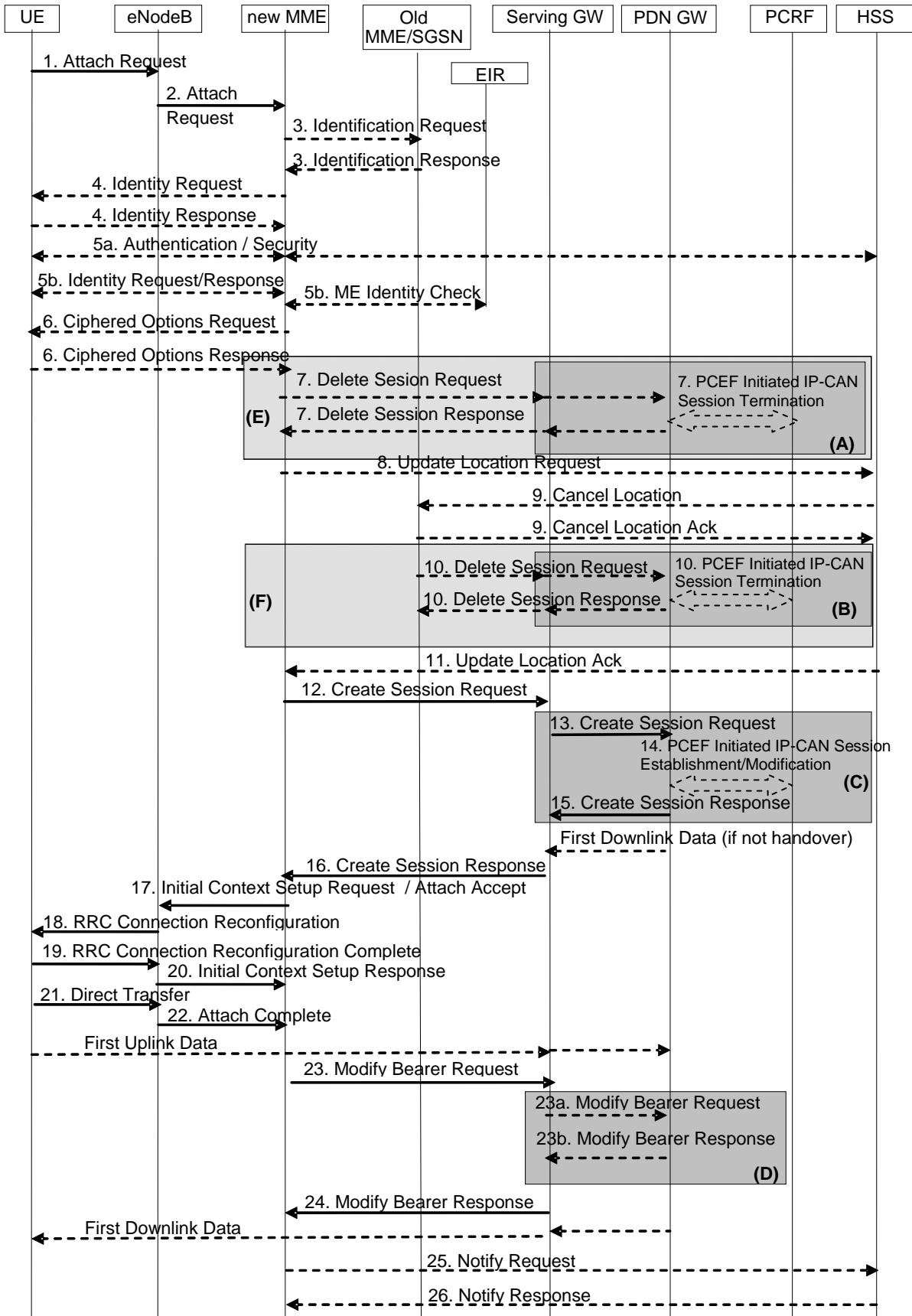
Figure 5.3.2.1-1: Attach procedure
