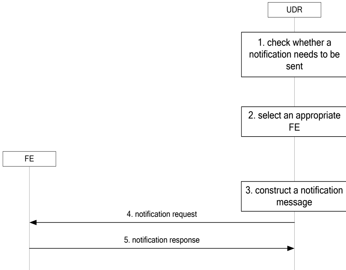
Figure 5.8-1: Notification procedure
