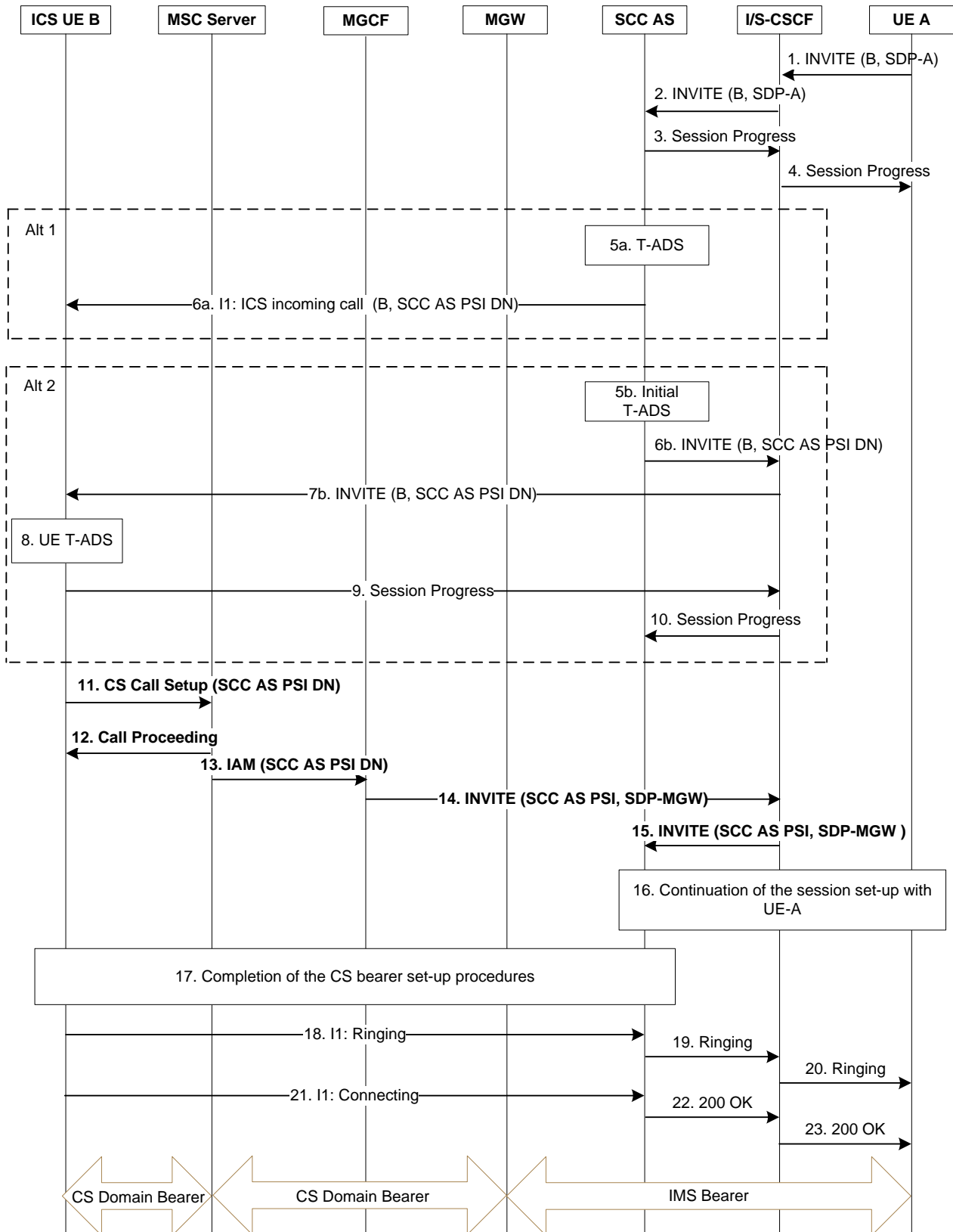
Figure 7.4.2.3-2: ICS UE Terminations with CS media information flows using I1 reference point when using an MSC Server
