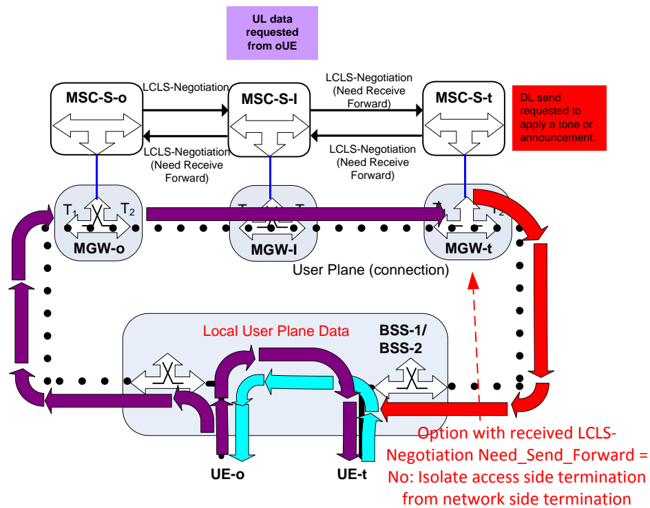
Figure A.2.2: iMSC requesting UL data from oUE and tMSC requesting DL data to tUE: option i isolate access side termination from network side termination
