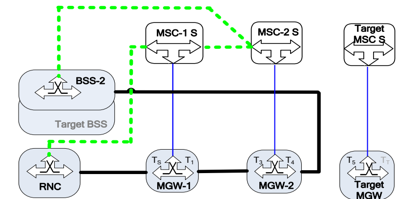
Connection Model 1: Before Handover
