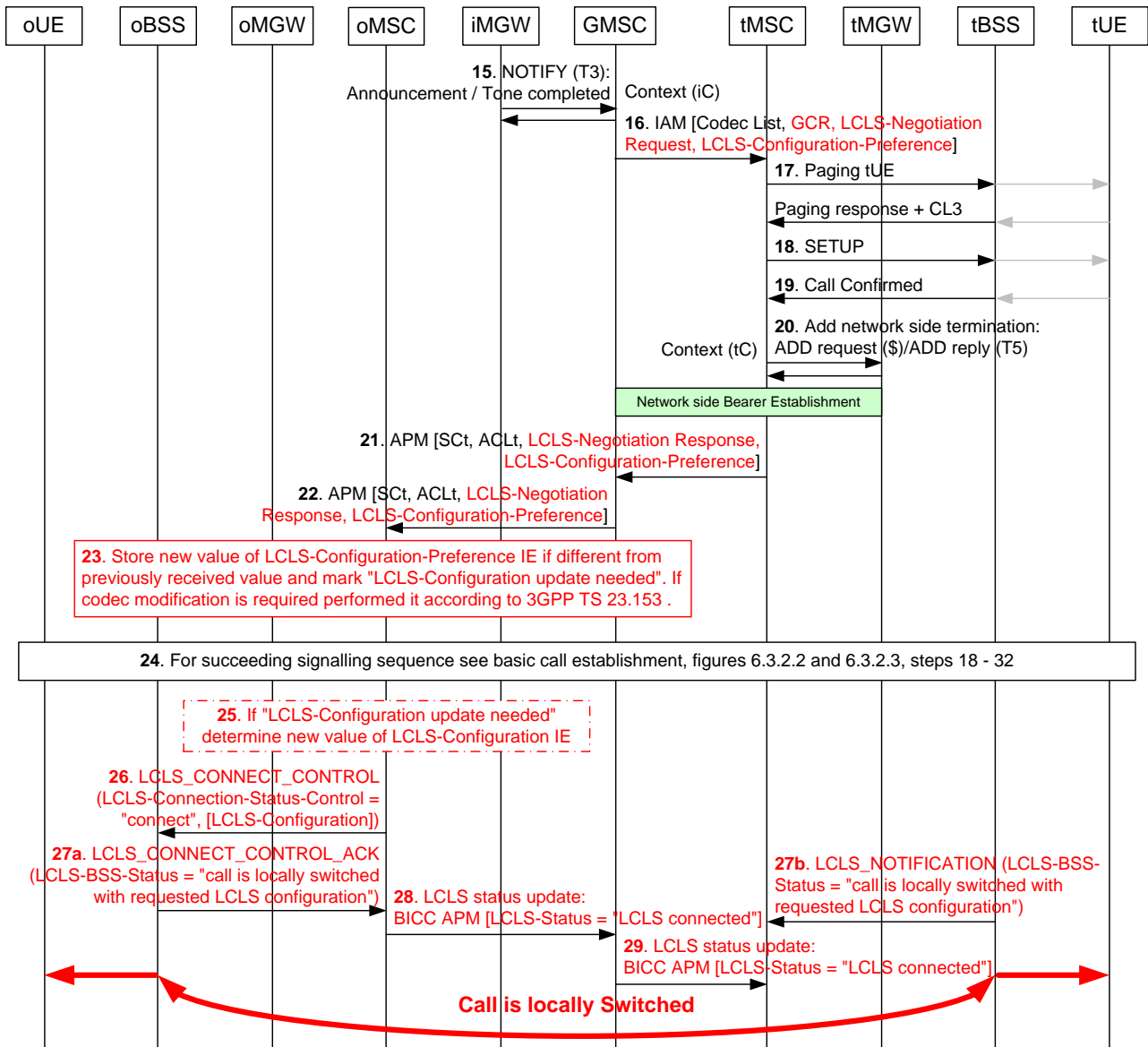
Figure 13.4.2.5.2: CFU, Call Establishment Flow (continuation of figure 13.4.2.5.1)
