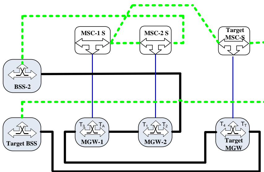
Connection Model 6: Handover completed, T_S termination was removed
