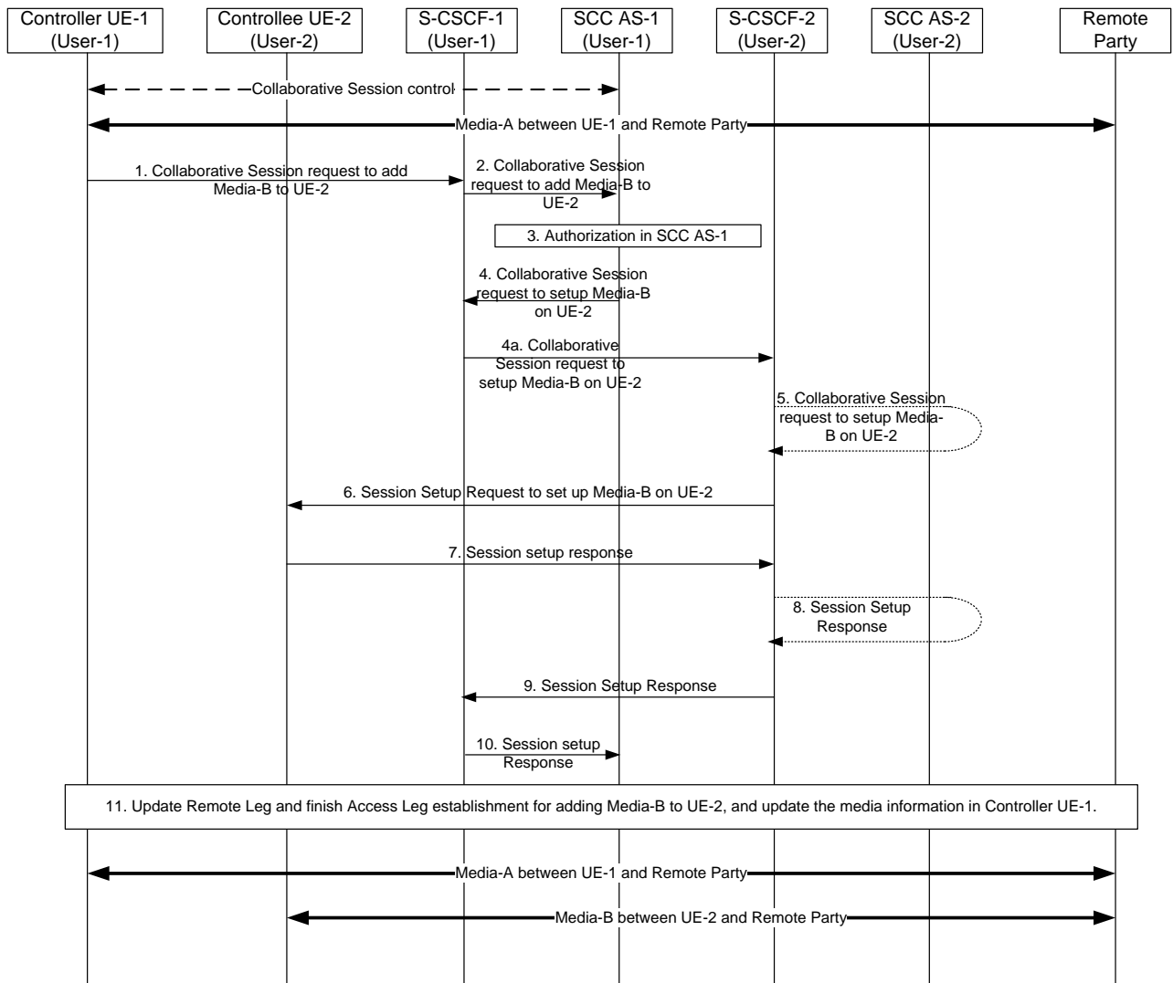
Figure 6a.4.2.2-1: Adding media by Controller UE to Controllee UE belonging to different IMS subscription
