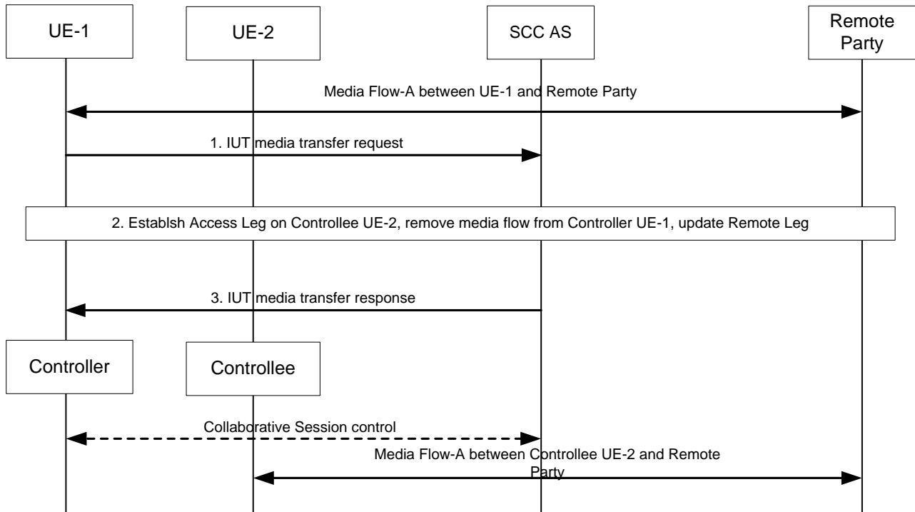
Figure 6a.2.1-1: Establish Collaborative Session by transferring media
