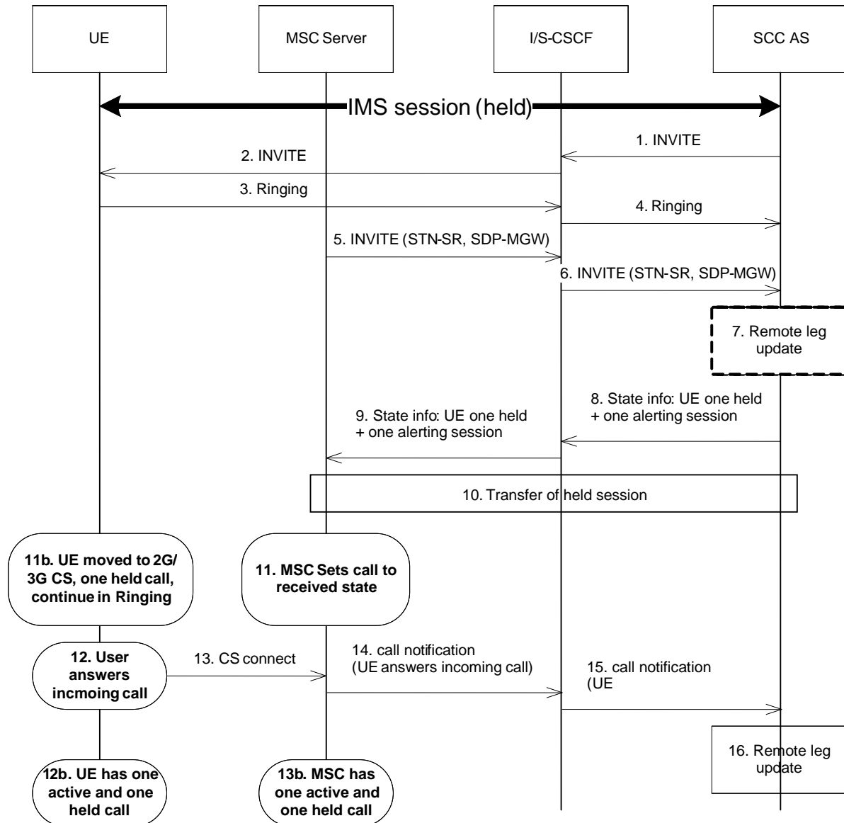
Figure 6.3.2.1.7c-1: PS-CS: PS to CS - Single Radio, mid-call service with an incoming call in alerting phase
