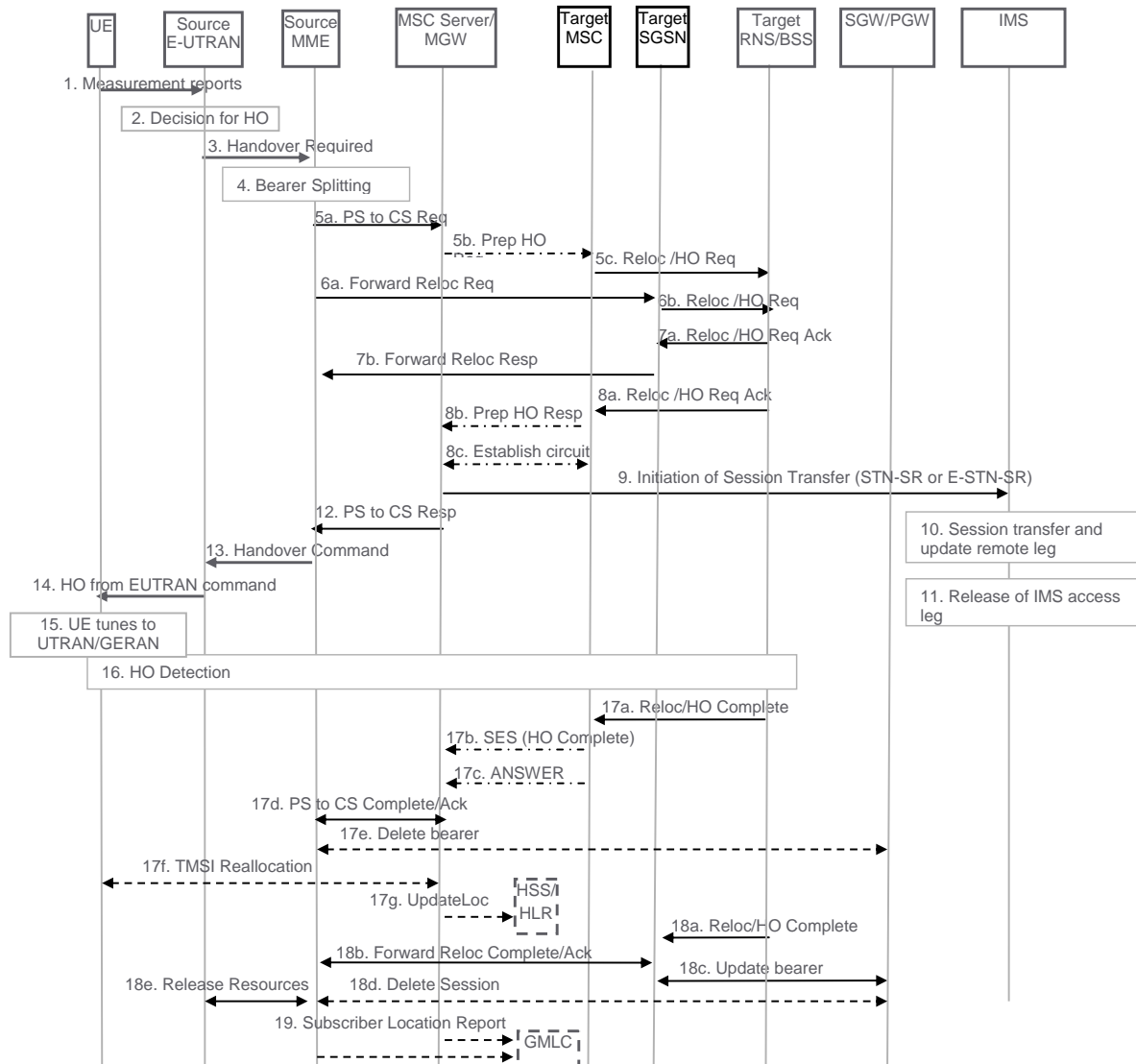
Figure 6.2.2.1-1: SRVCC from E-UTRAN to UTRAN with PS HO or GERAN with DTM HO support
