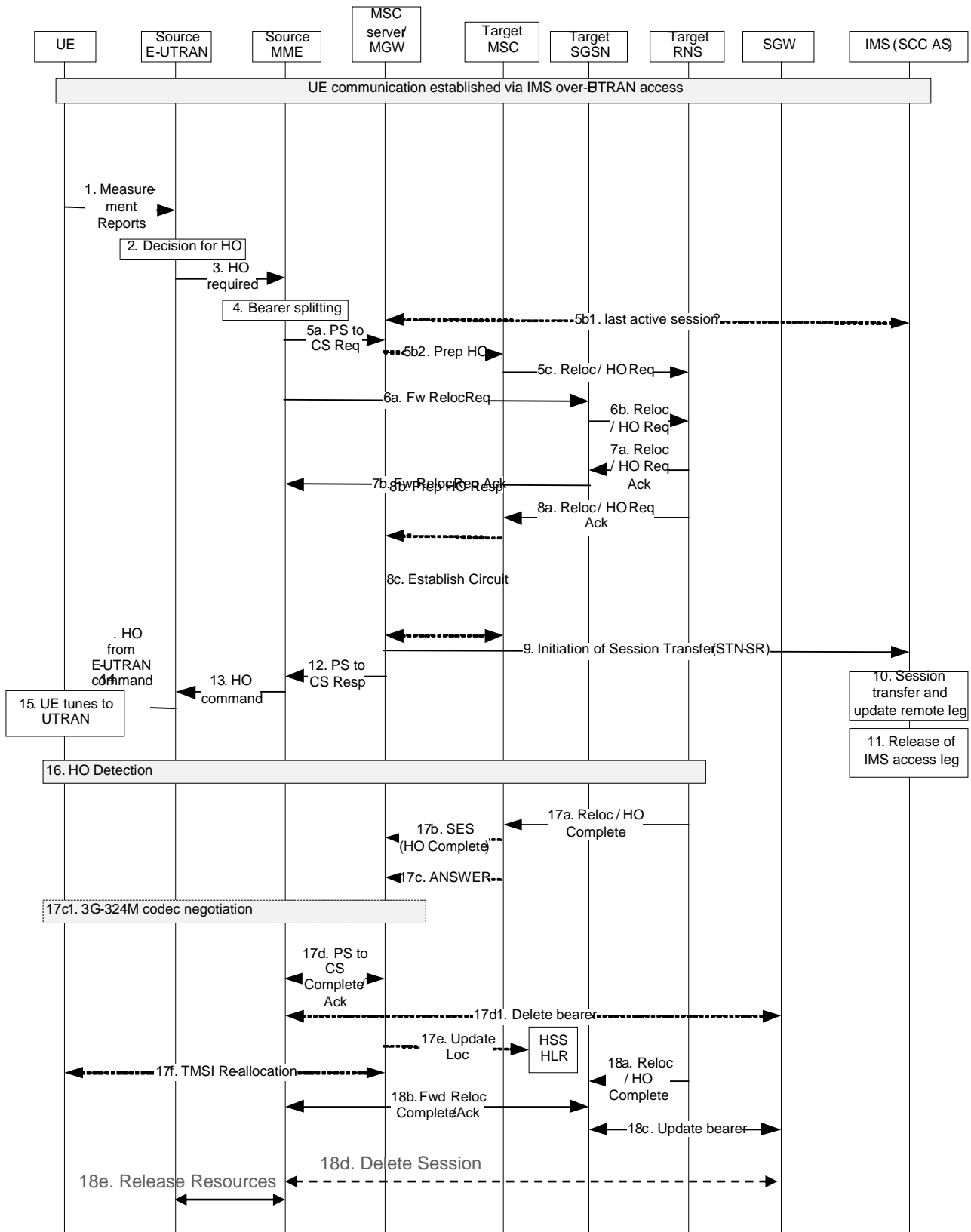
Figure 6.2.2.3-1: vSRVCC handover procedure
