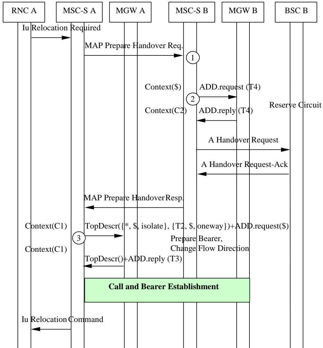
Figure 8.10/1: Basic Inter-MSC UMTS to GSM Handover (message sequence chart)
