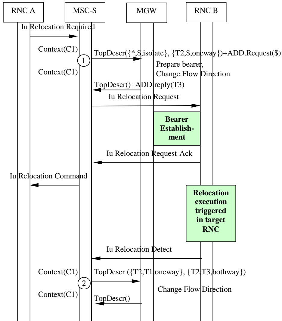
Figure 8.2/1: Intra-MSR SRNS Relocation (message sequence chart)
