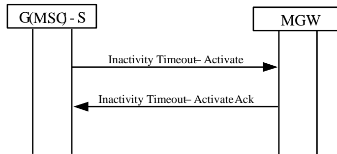
Figure 10.15.1: Inactivity Timeout - Activate
