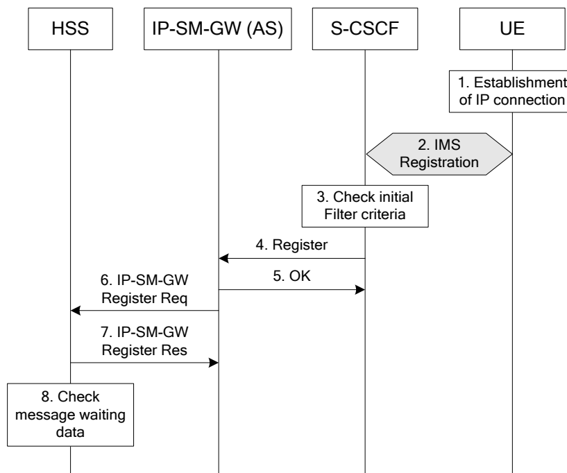
Figure 6.1: Registration procedure
