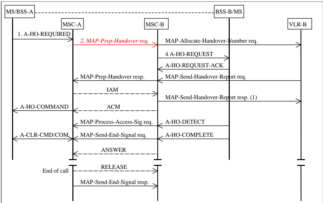
Figure 5.2.10-1. GSM to GSM inter-MSC handover
