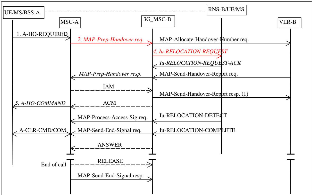
Figure 5.2.9-1: A/Gb mode to Iu mode inter-MSC handover
