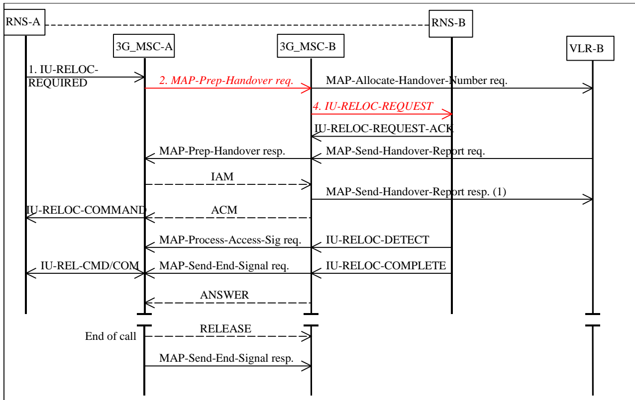
Figure 5.2.12-1. Inter-MSC SRNS relocation
