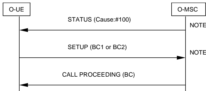
Figure 4.3: Fallback case
