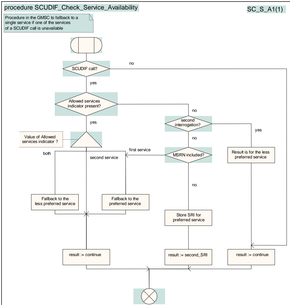
Figure 4.16J: Procedure SCUDIF_Check_Service_Availability
