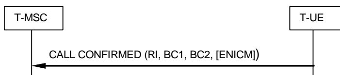
Figure 4.6: Normal case
