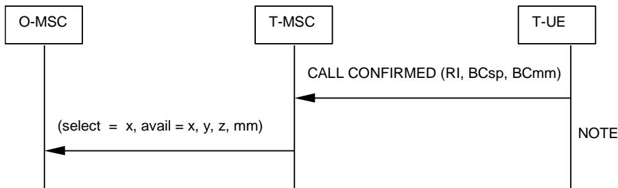
Figure 4.20: Multimedia only
