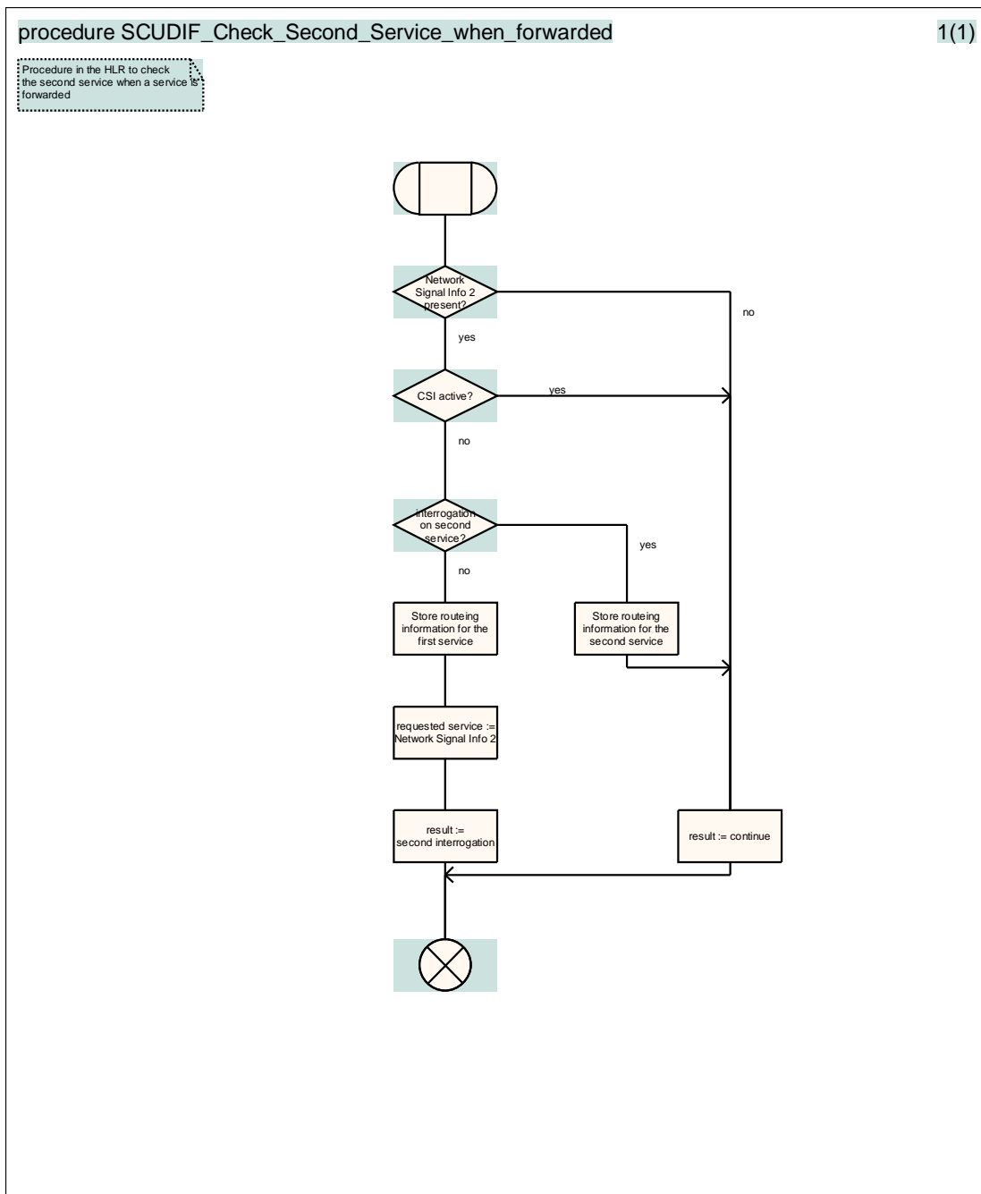
Figure 4.16H: Procedure SCUDIF_Check_Second_Service_when_Forwarded
