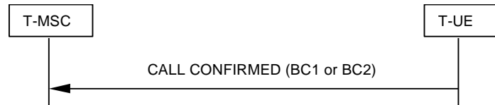
Figure 4.8: Fallback case
