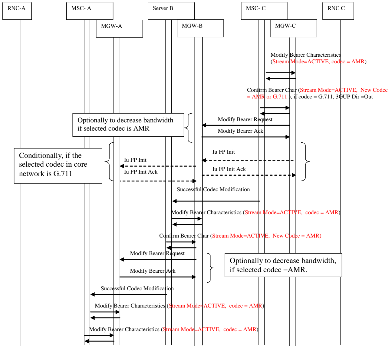
Figure 4.3.5.1/8: Network-initiated service change from MuMe to speech (continue)
