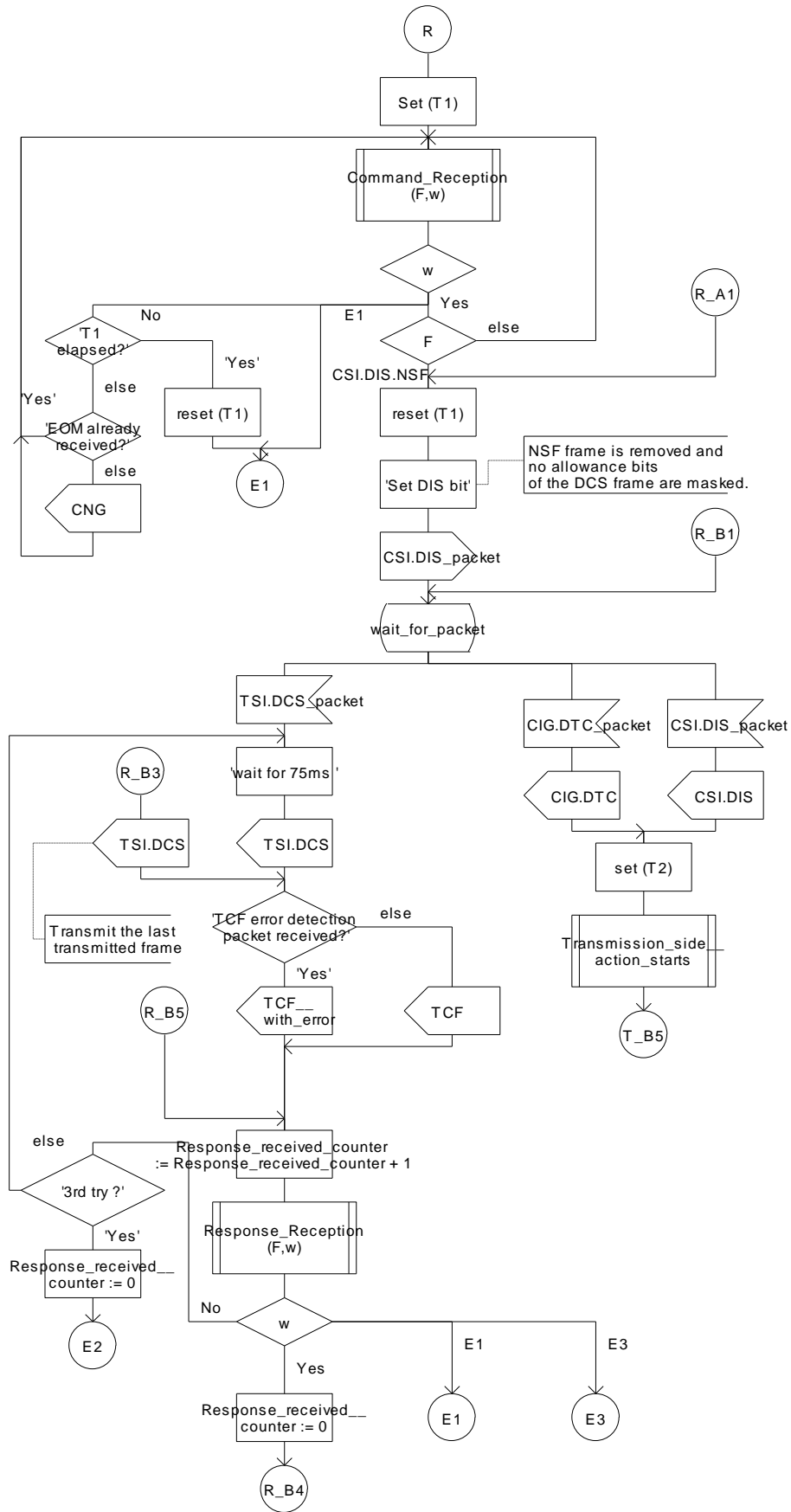
Figure D.5: Reception side FA, Phase B
