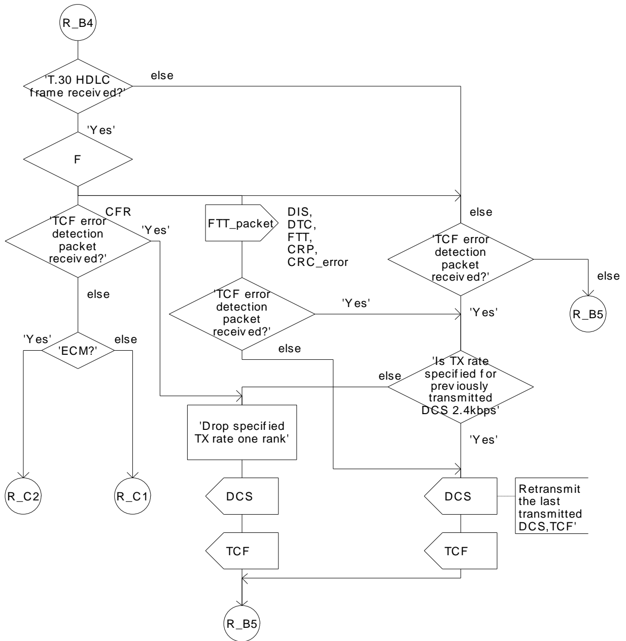
Figure D.9: Output conditions for FTT and specified TX rate decision algorithm for DCS NONECM & ECM
