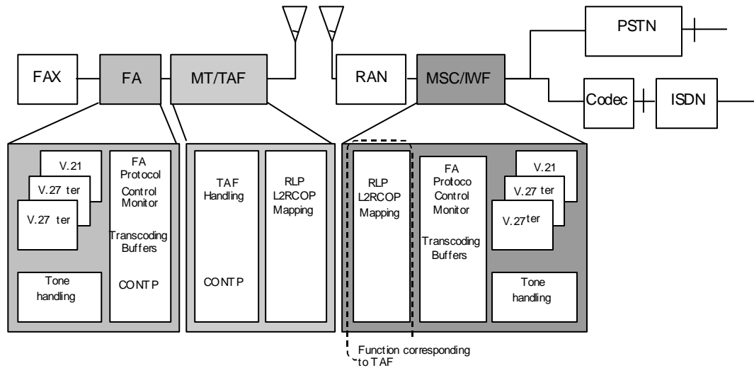
Figure 6: Network interworking
