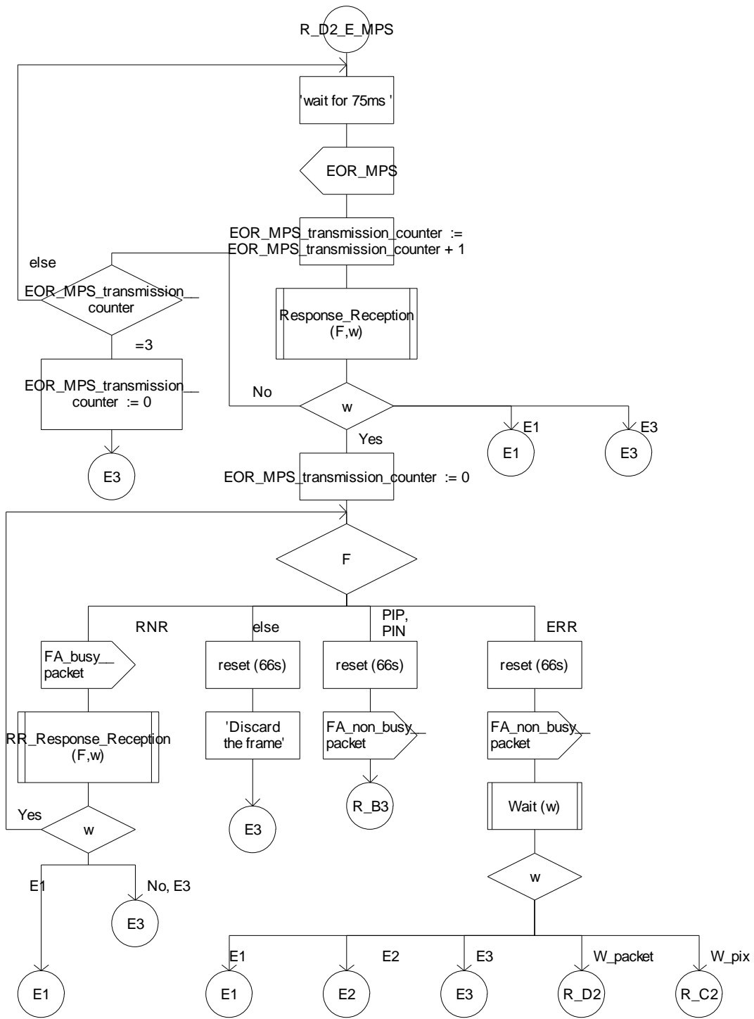
Figure D.28: Reception FA, Phase D (EOR-MPS)
