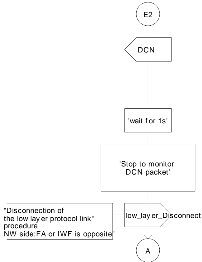
Figure D.36: FA release flow (2)
