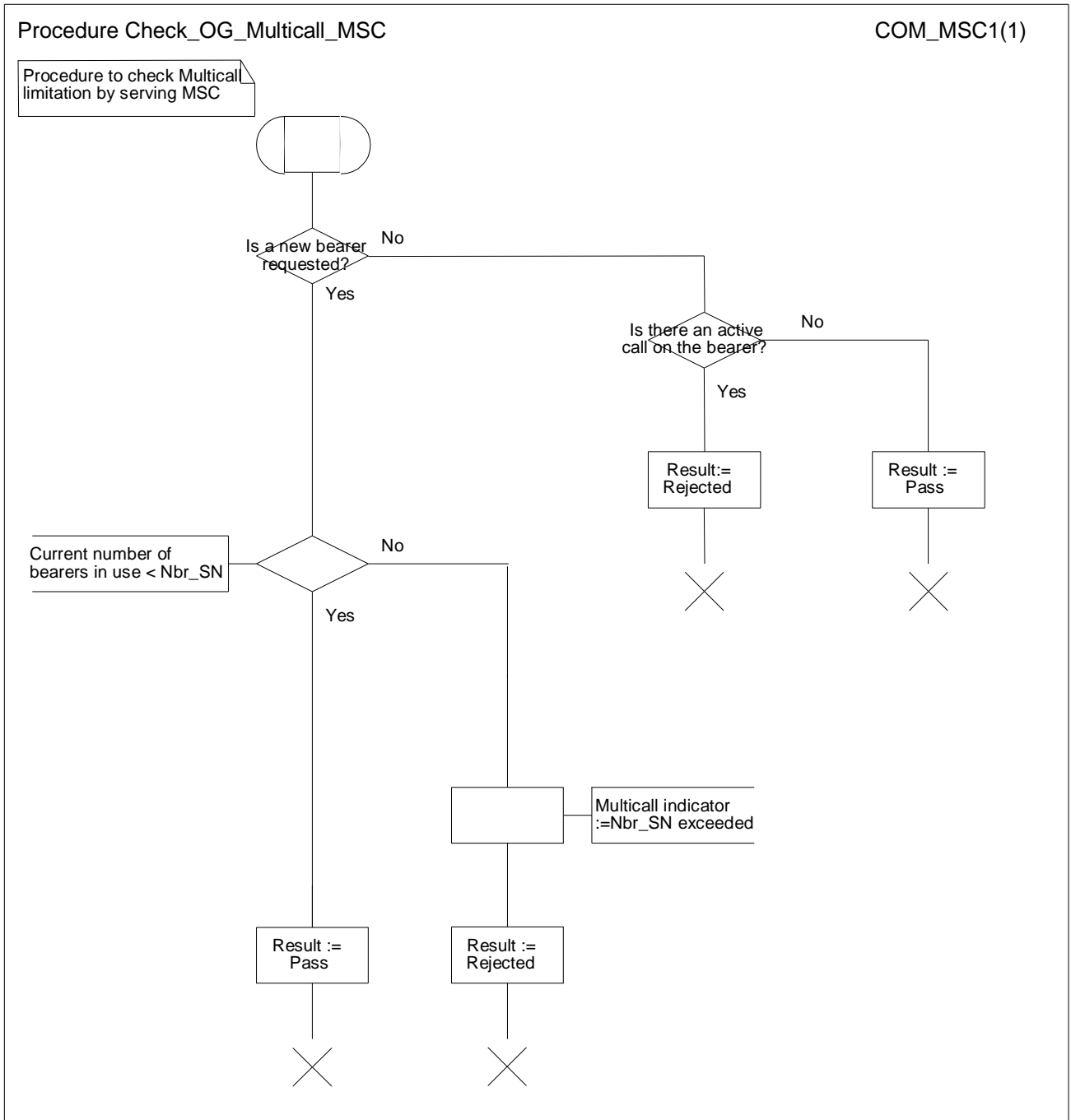
Figure 8: Procedure Check_OG_Multicall_MSC
