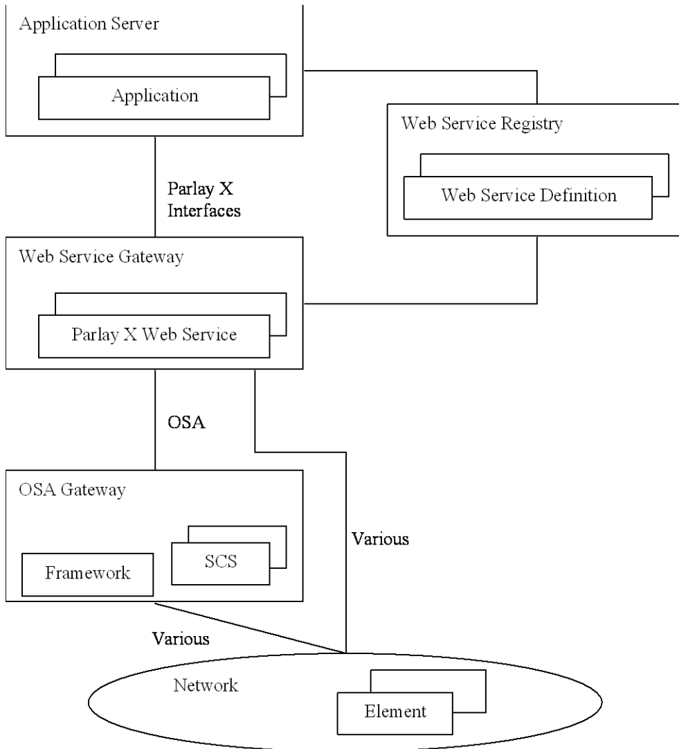
Figure 9.2 The overall Parlay X Web Services architecture
