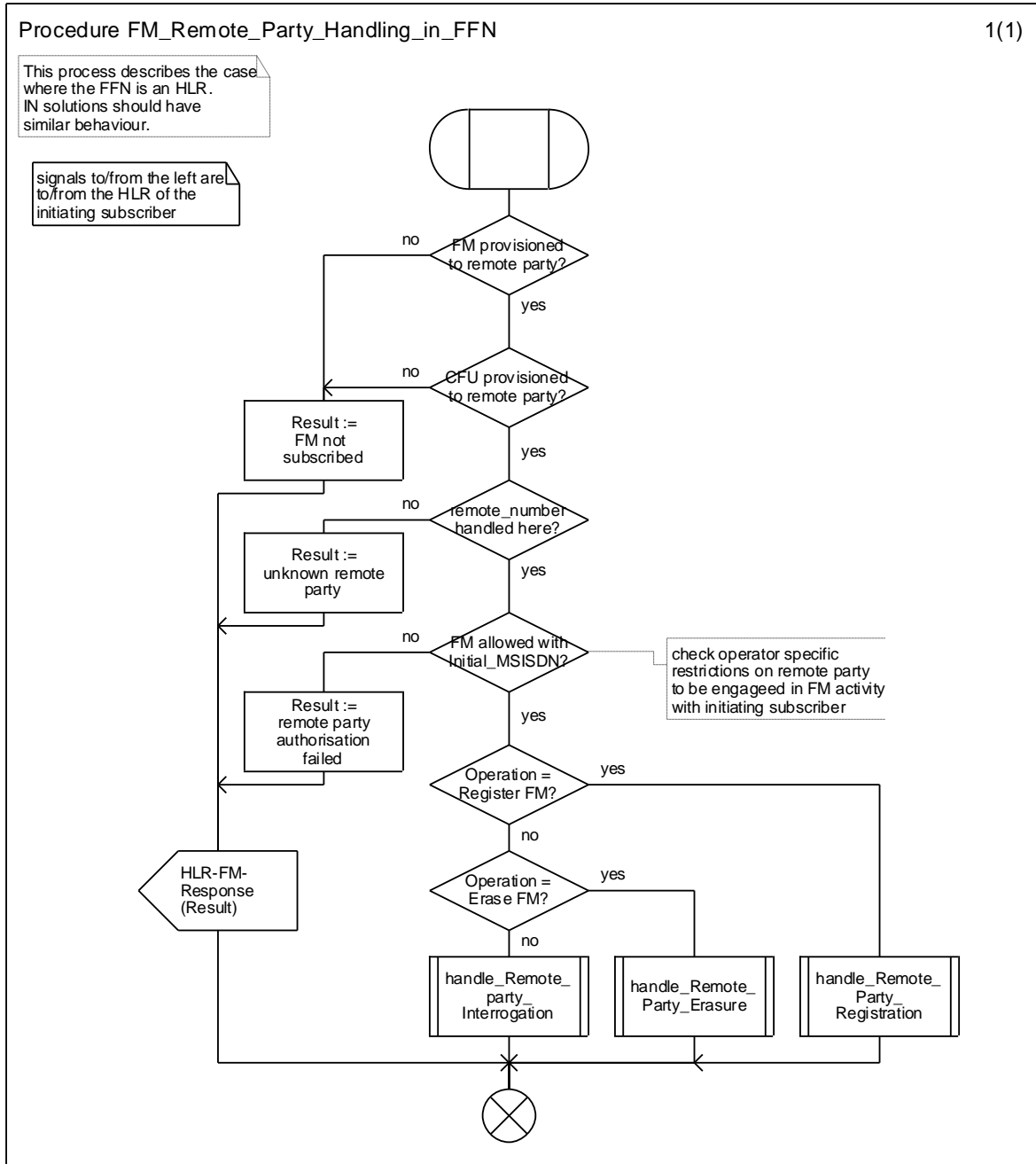
Figure 4.5: Procedure: FM_Remote_Party_Handling_in_FFN
