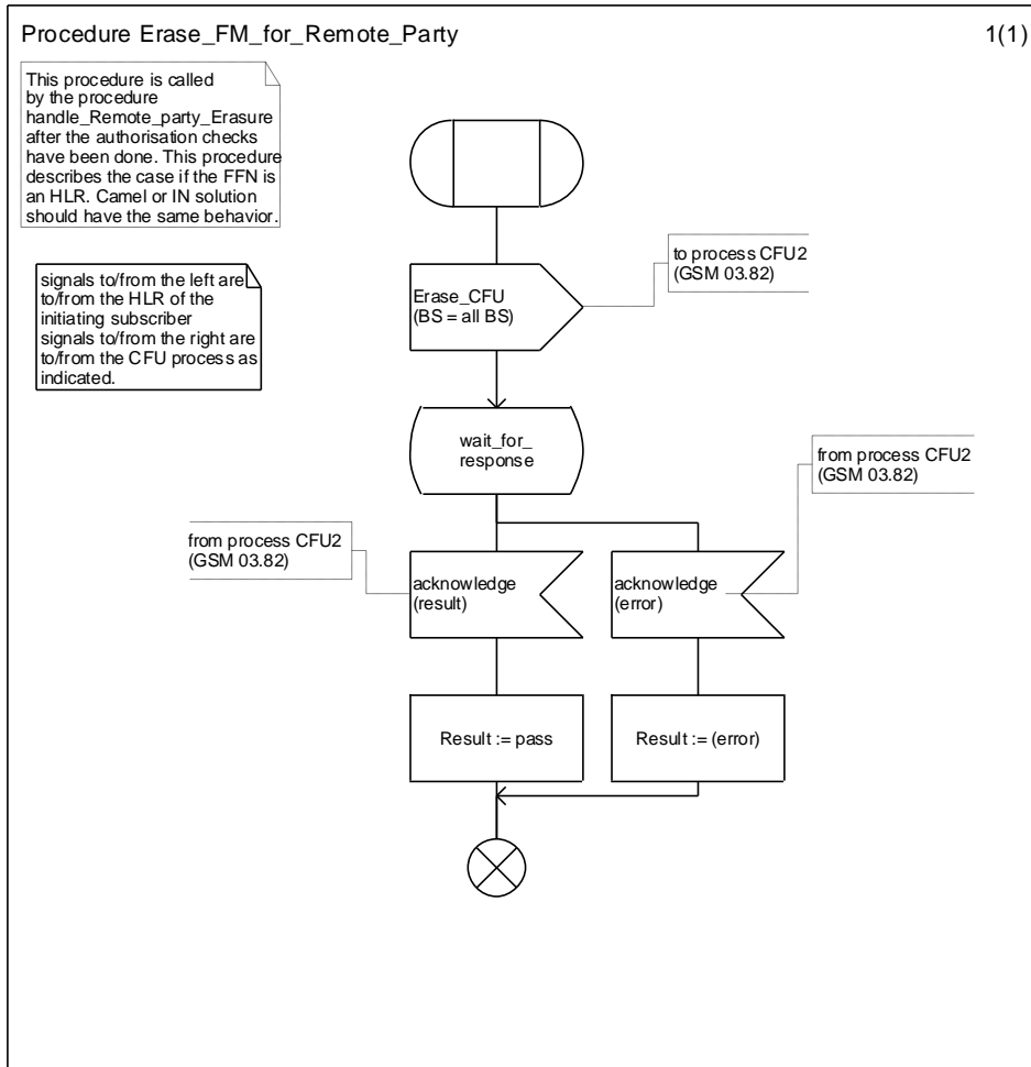
Figure 4.7a: Procedure Erase_FM_for_Remote_party
