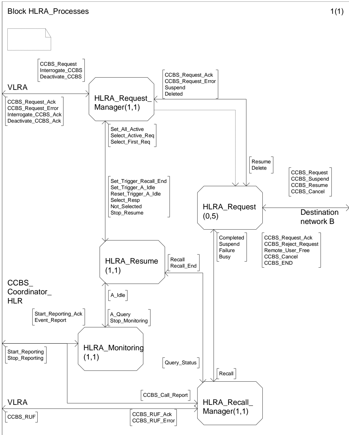
Figure 11.1.2.1: HLRA Processes
