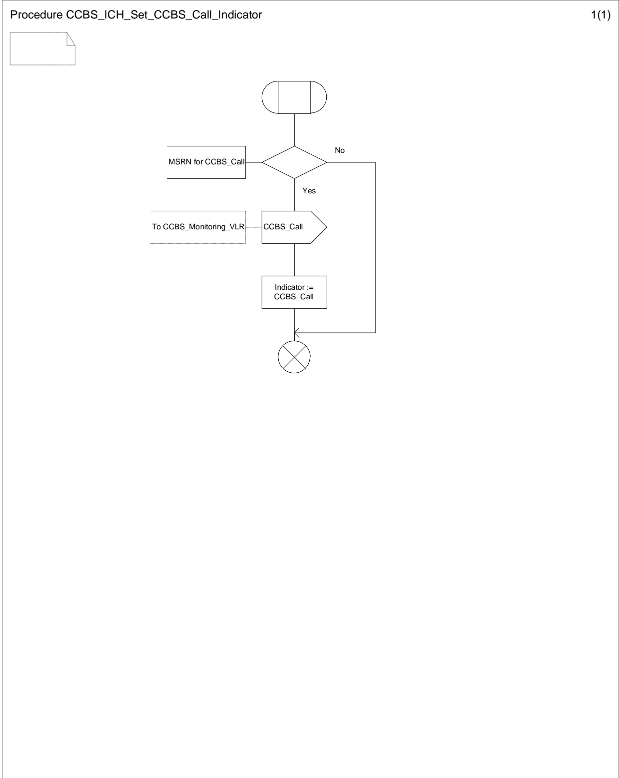
Figure 11.2.3.3: Procedure CCBS_ICH_Set_CCBS_Call_Indicator
