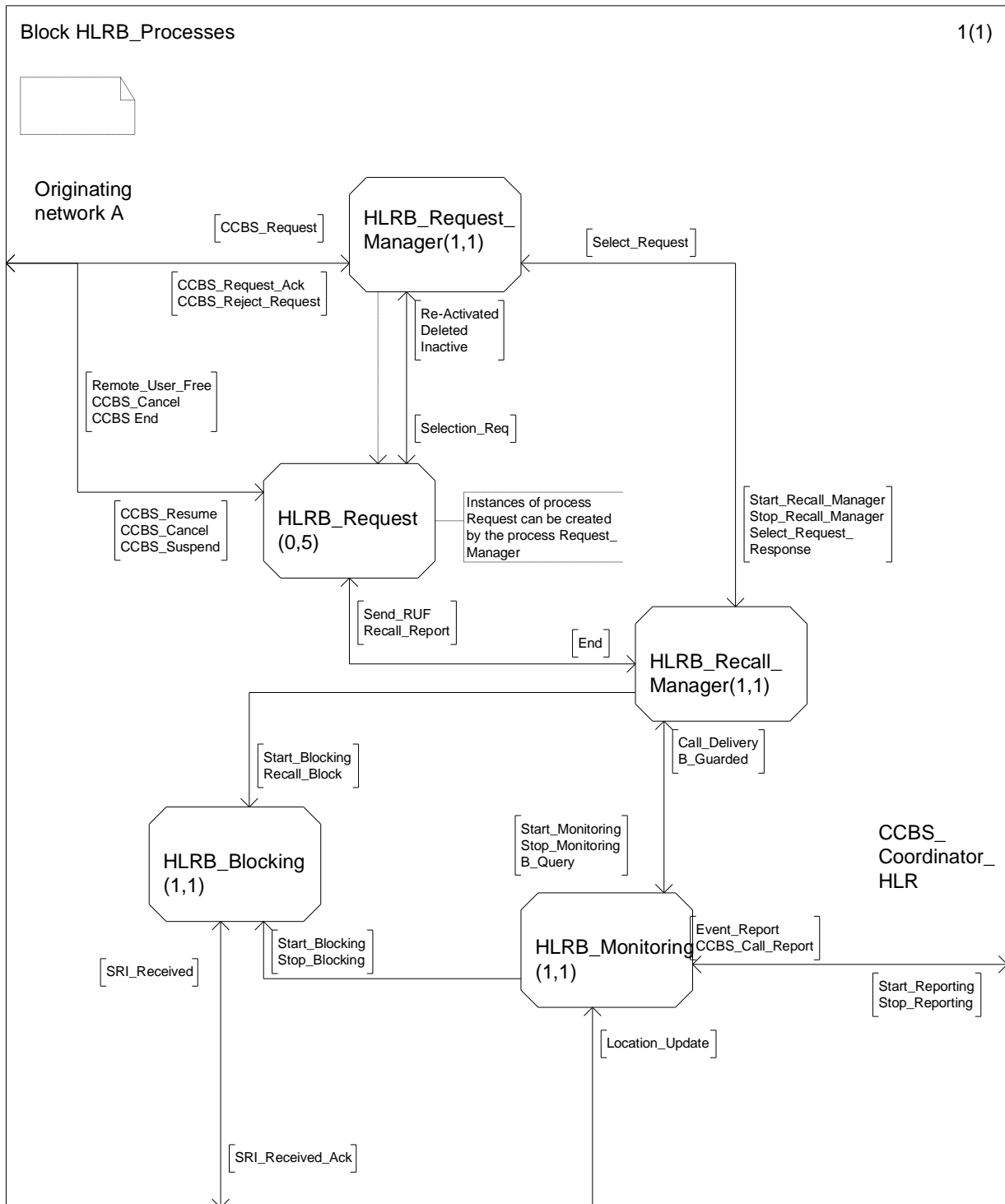
Figure 11.2.2.1: HLRB_Processes
