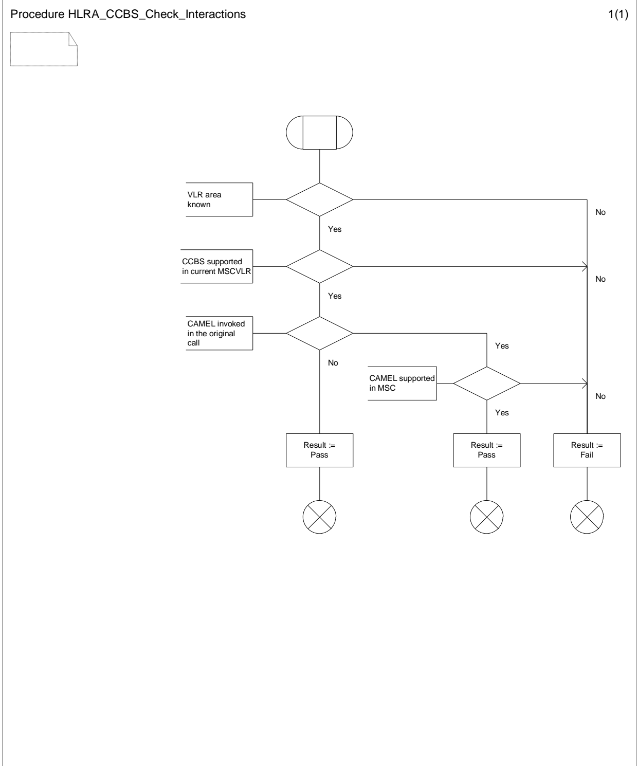
Figure 11.1.2.7: Procedure HLRA_CCBS_Check_Interactions
