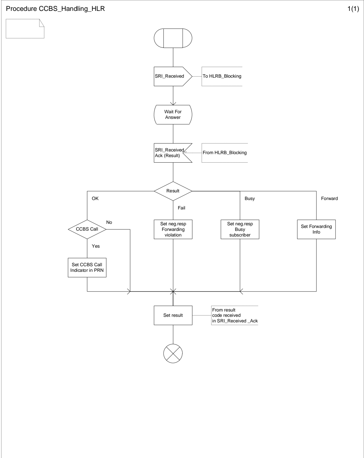
Figure 11.2.2.8: Procedure CCBS_Handling_HLR
