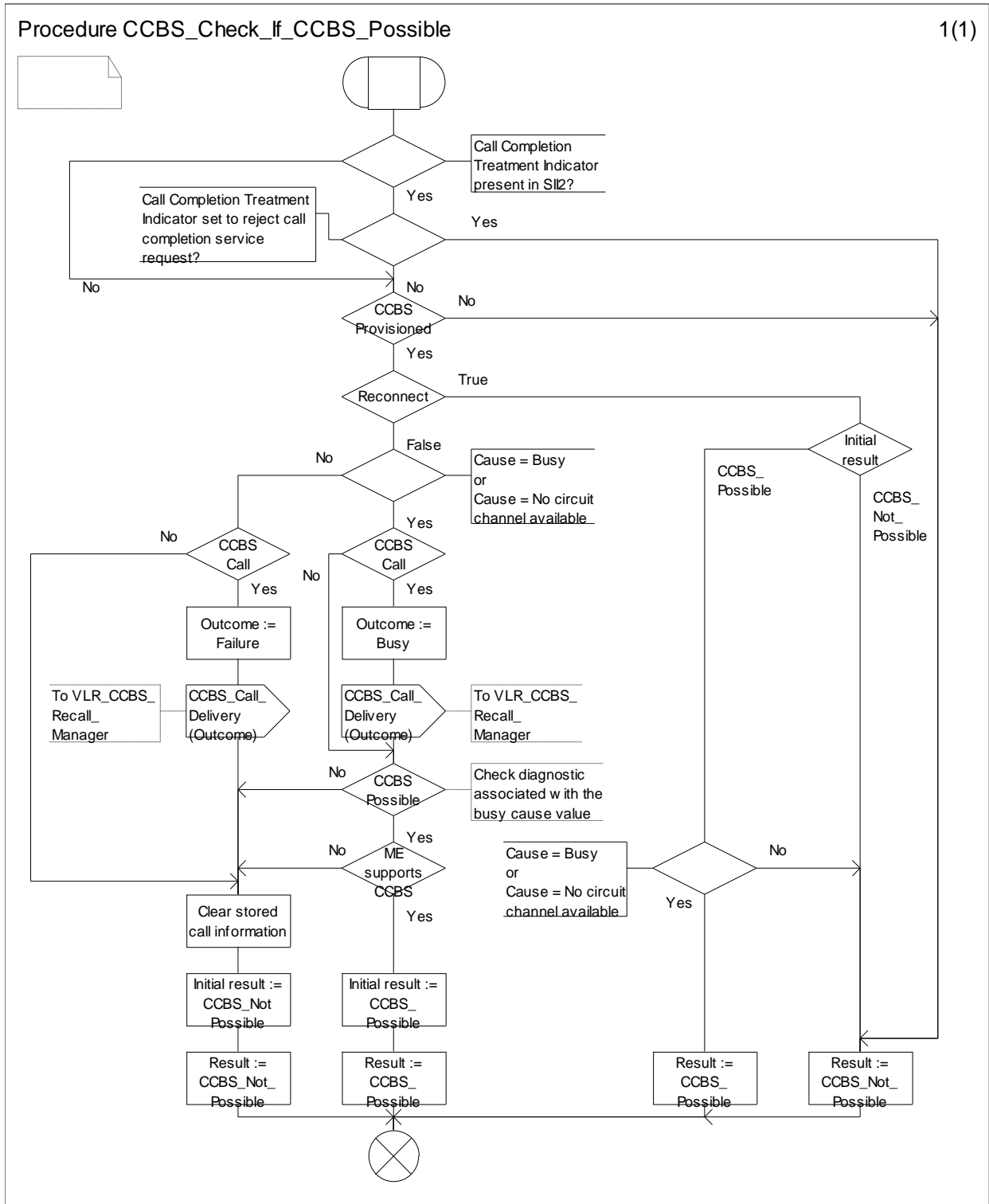
Figure 11.1.1.5: Procedure CCBS_Check_If_CCBS_Possible
