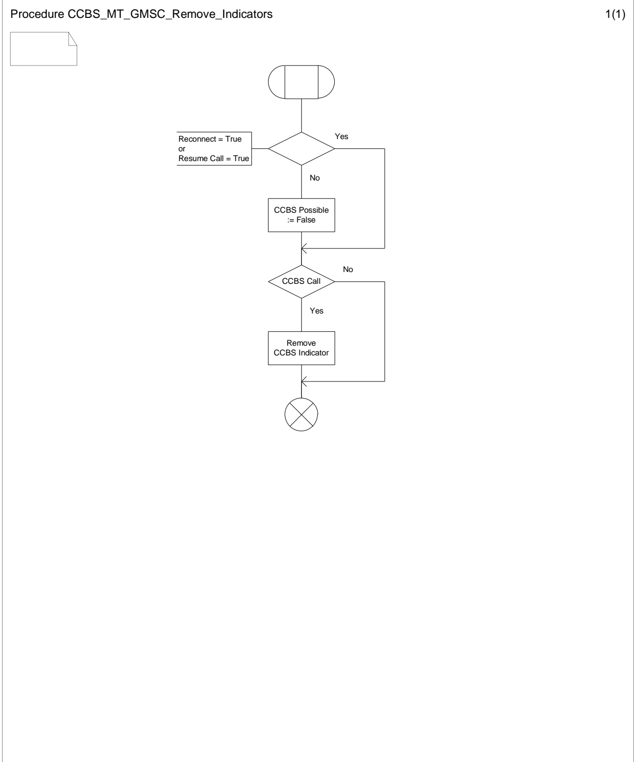
Figure 11.2.1.4: Procedure CCBS_MT_GMSC_Remove_Indicators
