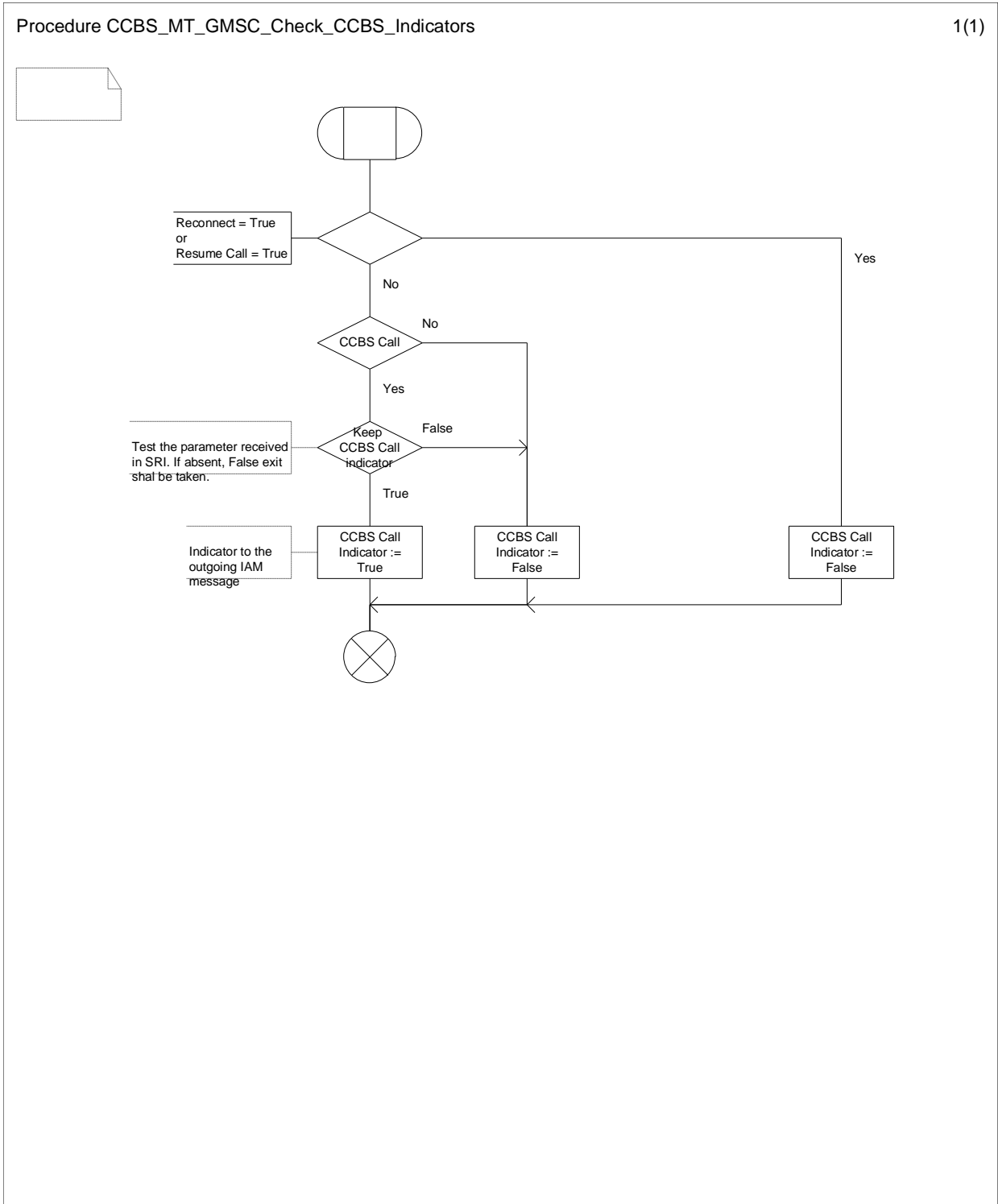
Figure 11.2.1.2: Procedure CCBS_MT_GMSC_Check_CCBS_Indicators
