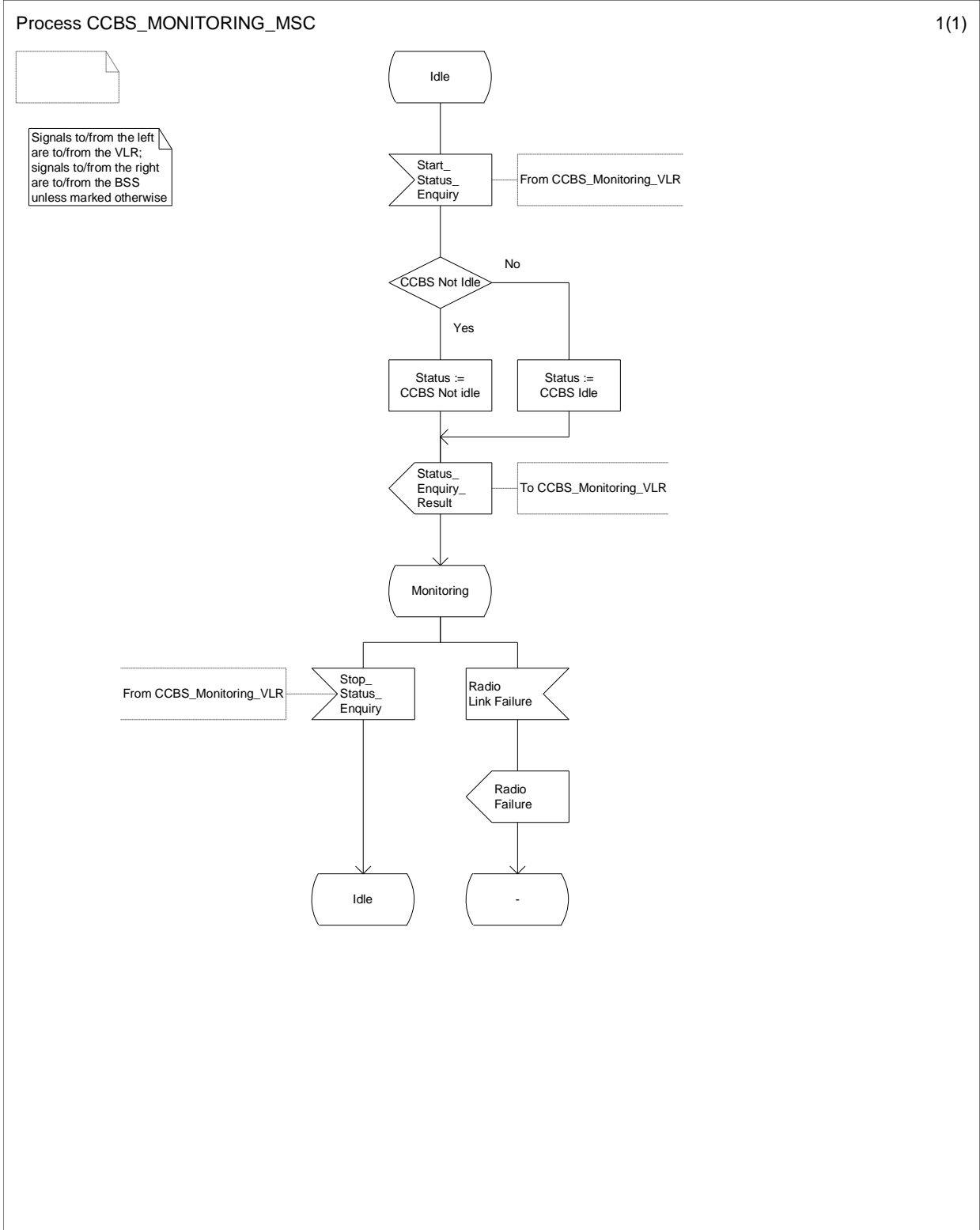
Figure 11.3.2: Process CCBS_Monitoring_MSC
