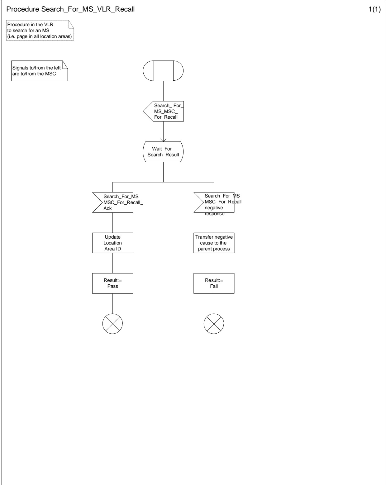
Figure 11.1.1.9: Procedure Search_For_MS_VLR_Recall
