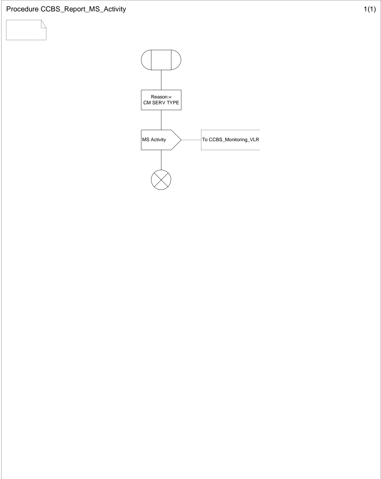
Figure 11.3.6: Procedure CCBS_Report_MS_Activity
