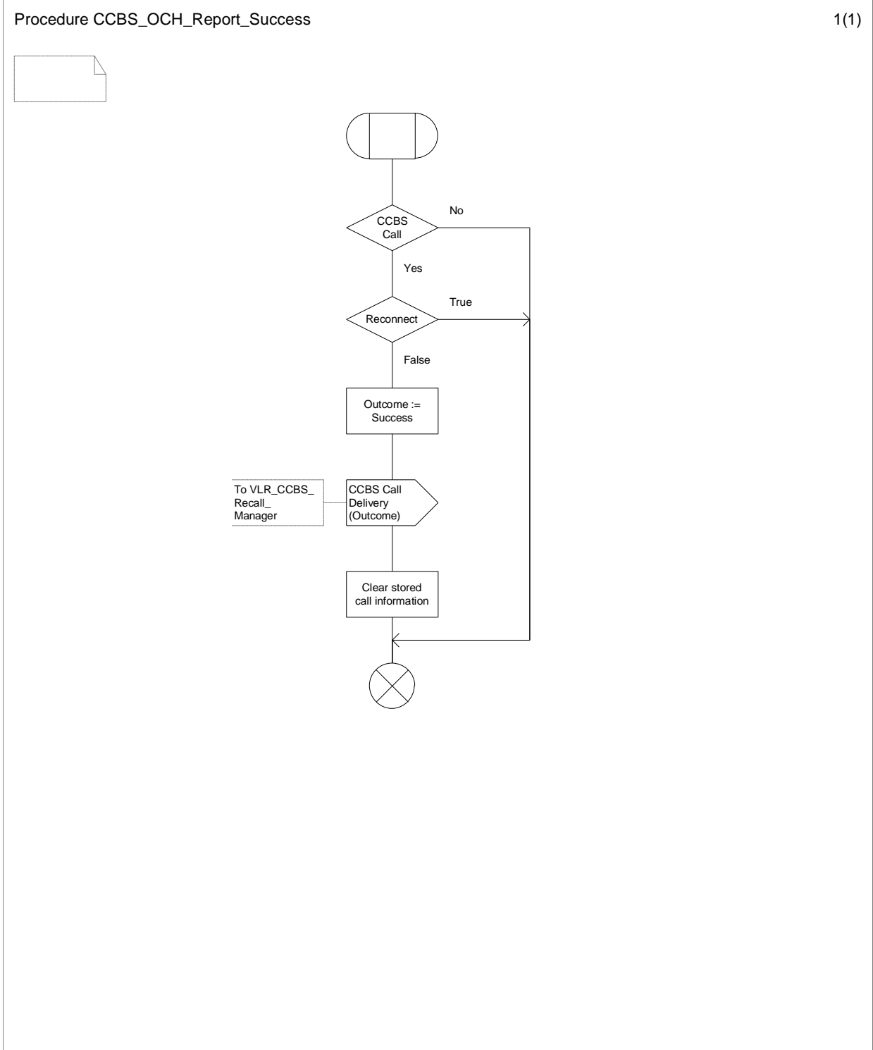
Figure 11.1.1.11: Procedure CCBS_OCH_Report_Success
