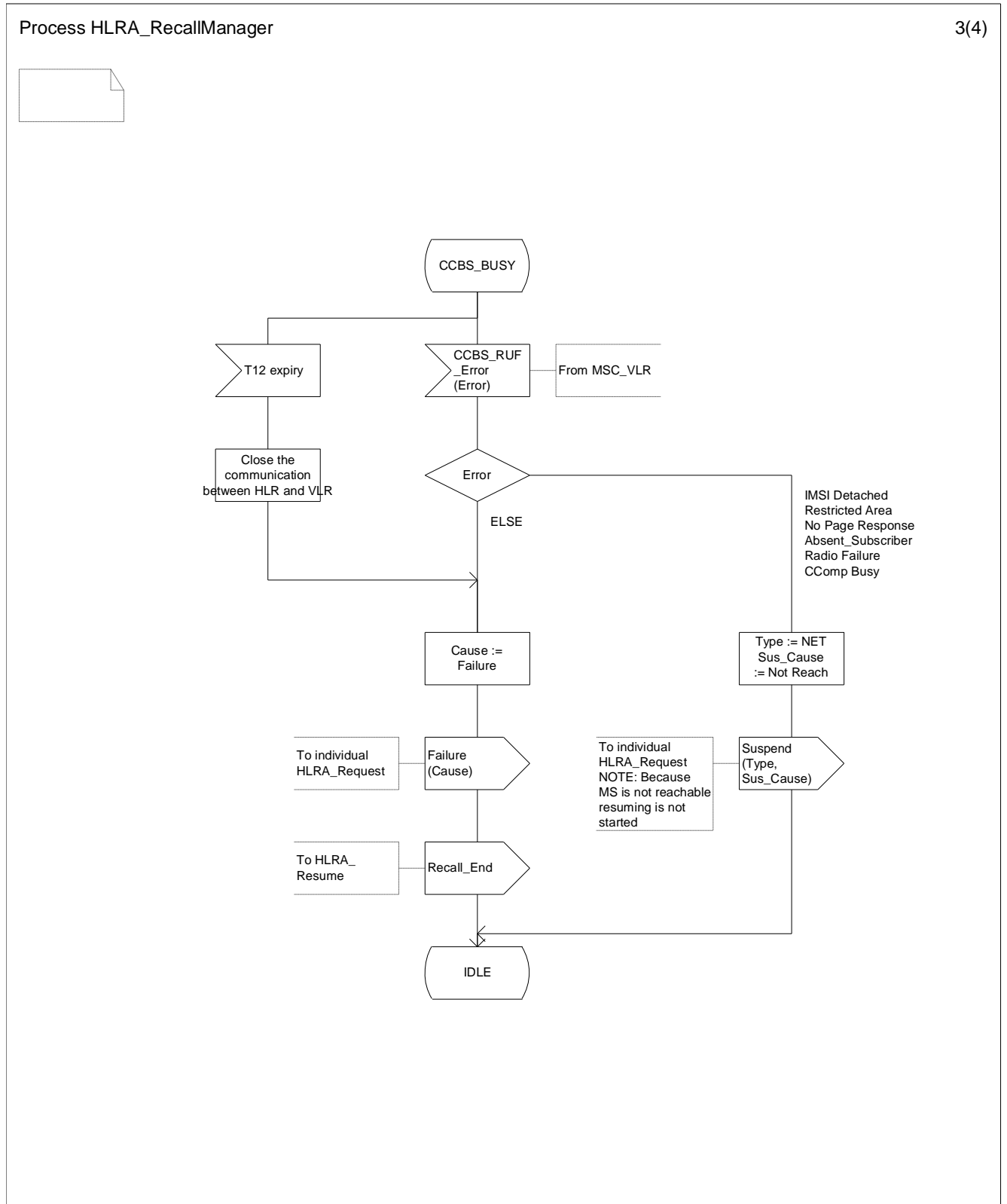
Figure 11.1.2.4: Process HLRA_Recall_Manager (sheet 3 of 4)
