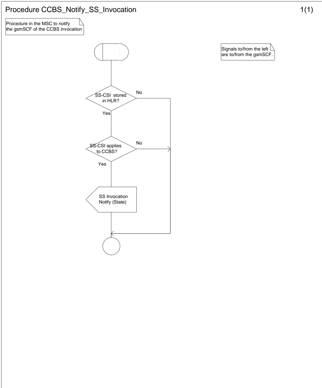
Figure 11.1.2.8: Procedure CCBS_Notify_SS_Invocation
