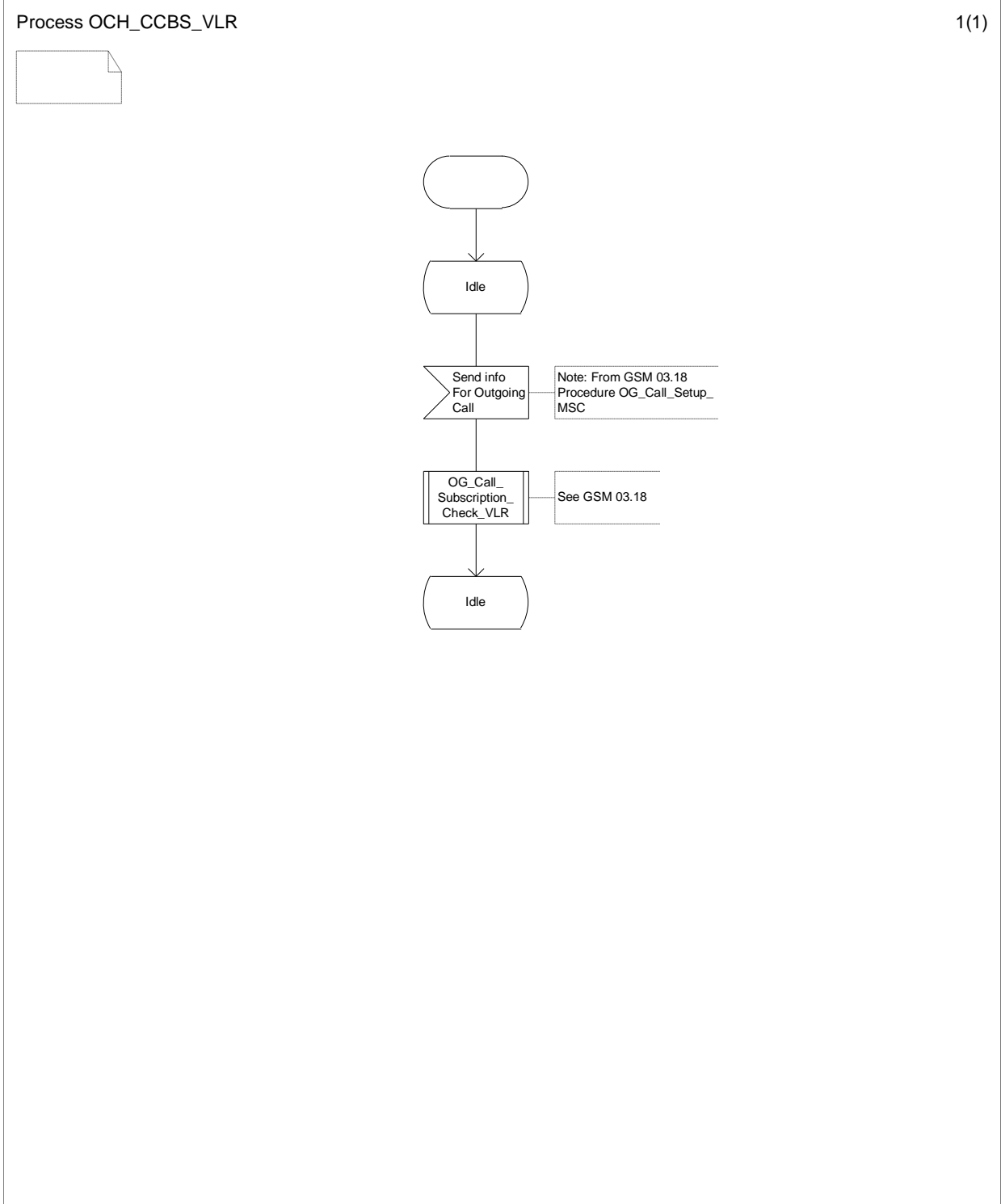
Figure 11.1.1.3: Process OCH_CCBS_VLR
