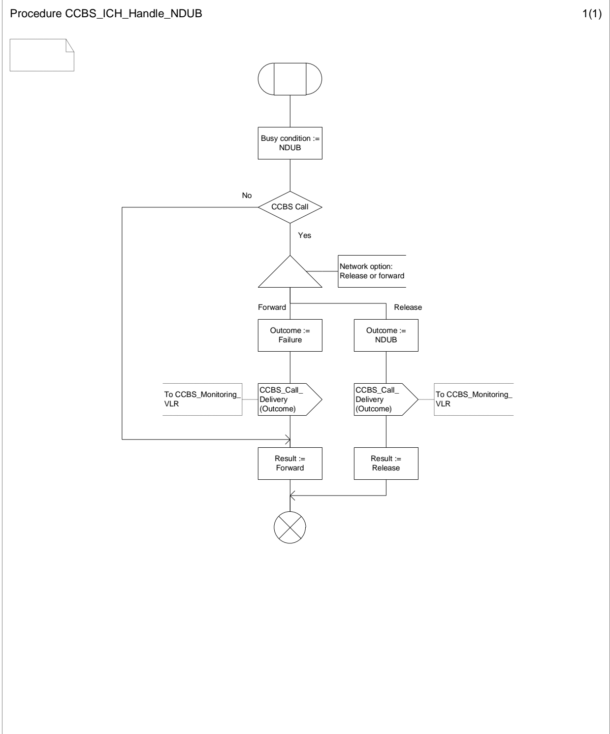
Figure 11.2.3.7: Procedure CCBS_ICH_Handle_NDUB
