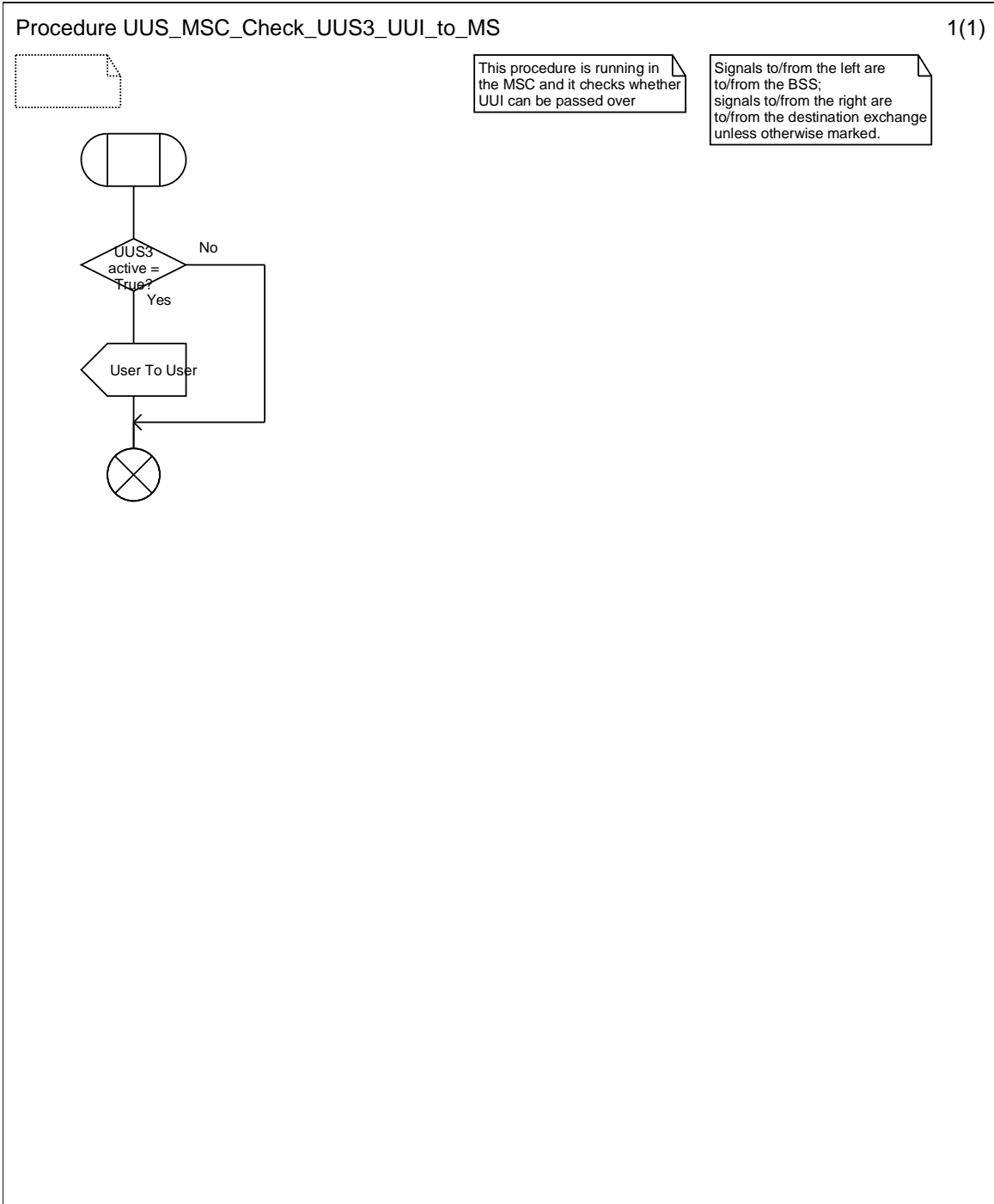
Figure 9.3.4: Procedure UUS_MSC_Check_UUS3_UUI_to_MS
