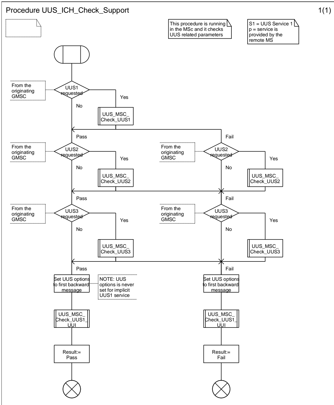
Figure 9.2.2.1: Procedure UUS_ICH_Check_Support
