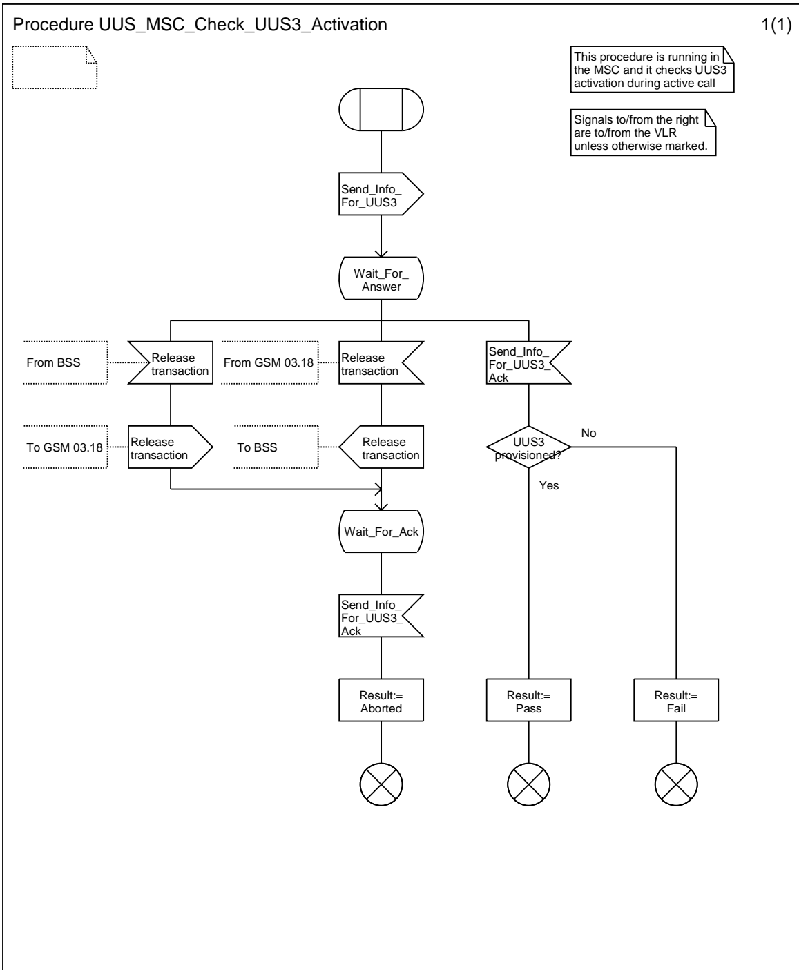
Figure 9.4.1.2: Procedure UUS_MSC_Check_UUS3_Activation
