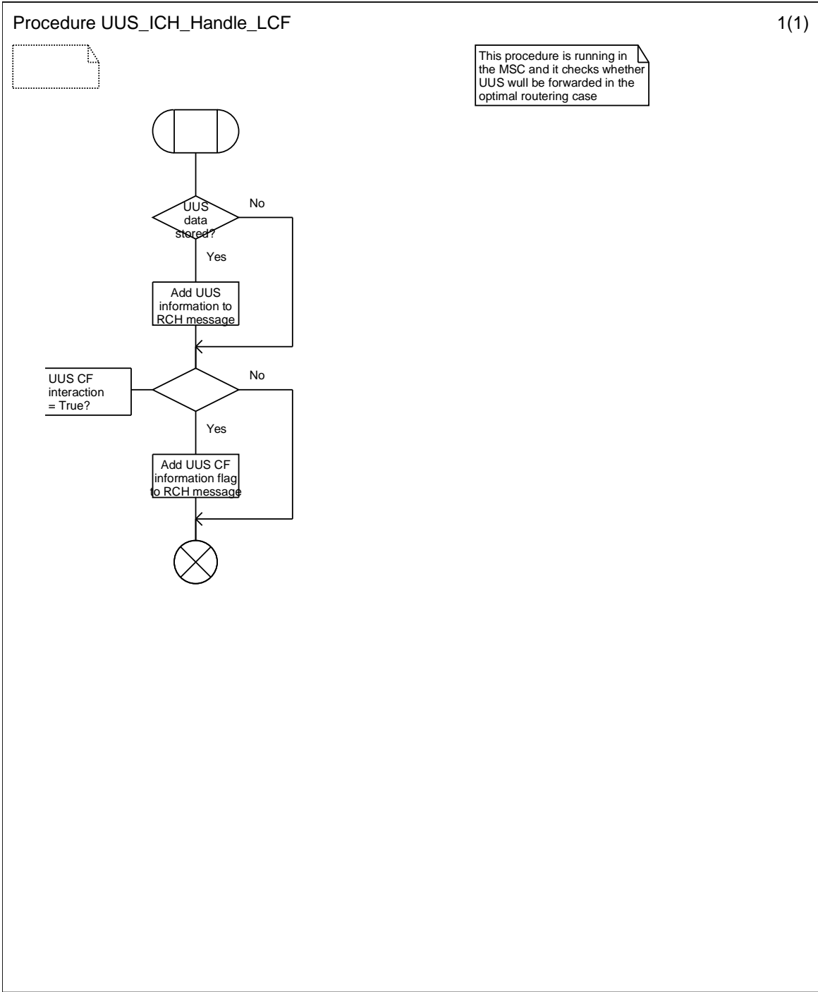
Figure 9.2.2.3: Procedure UUS_ICH_Handle_LCF
