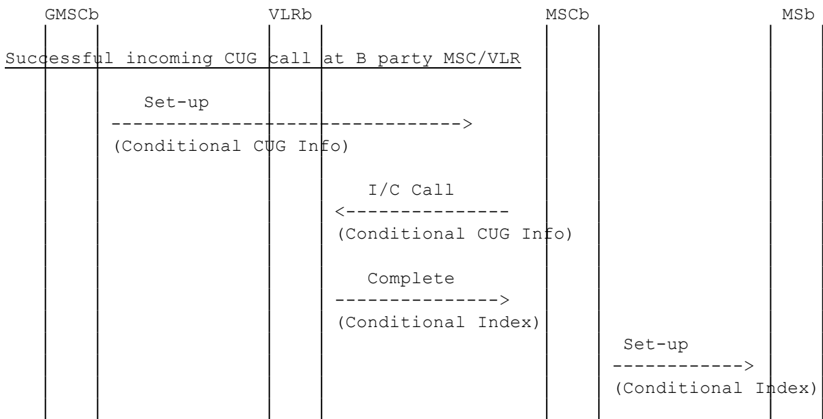
Figure 1.5: MT CUG call handling at called party MSC/VLR
