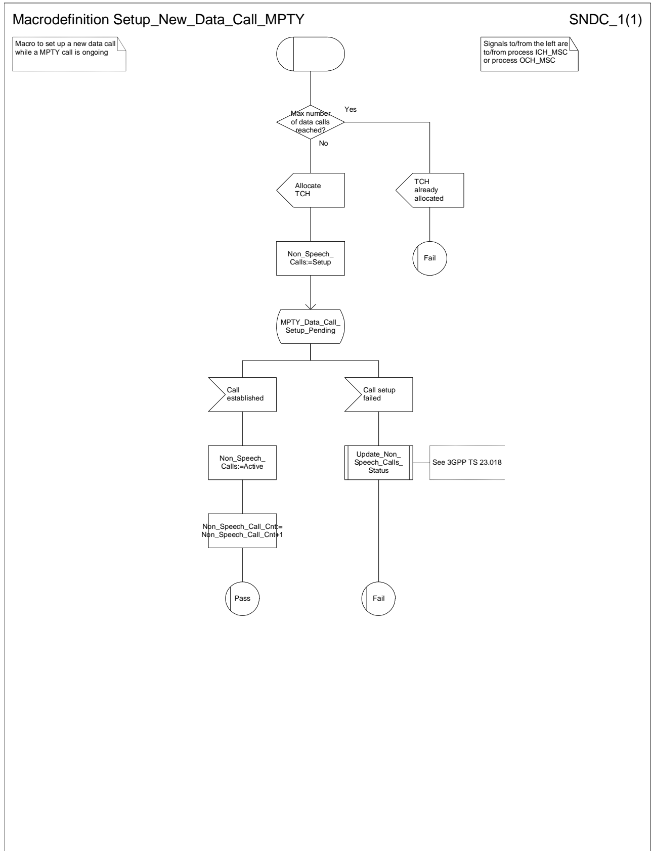
Figure 1.4: Setup_New_Data_Call_MPTY
