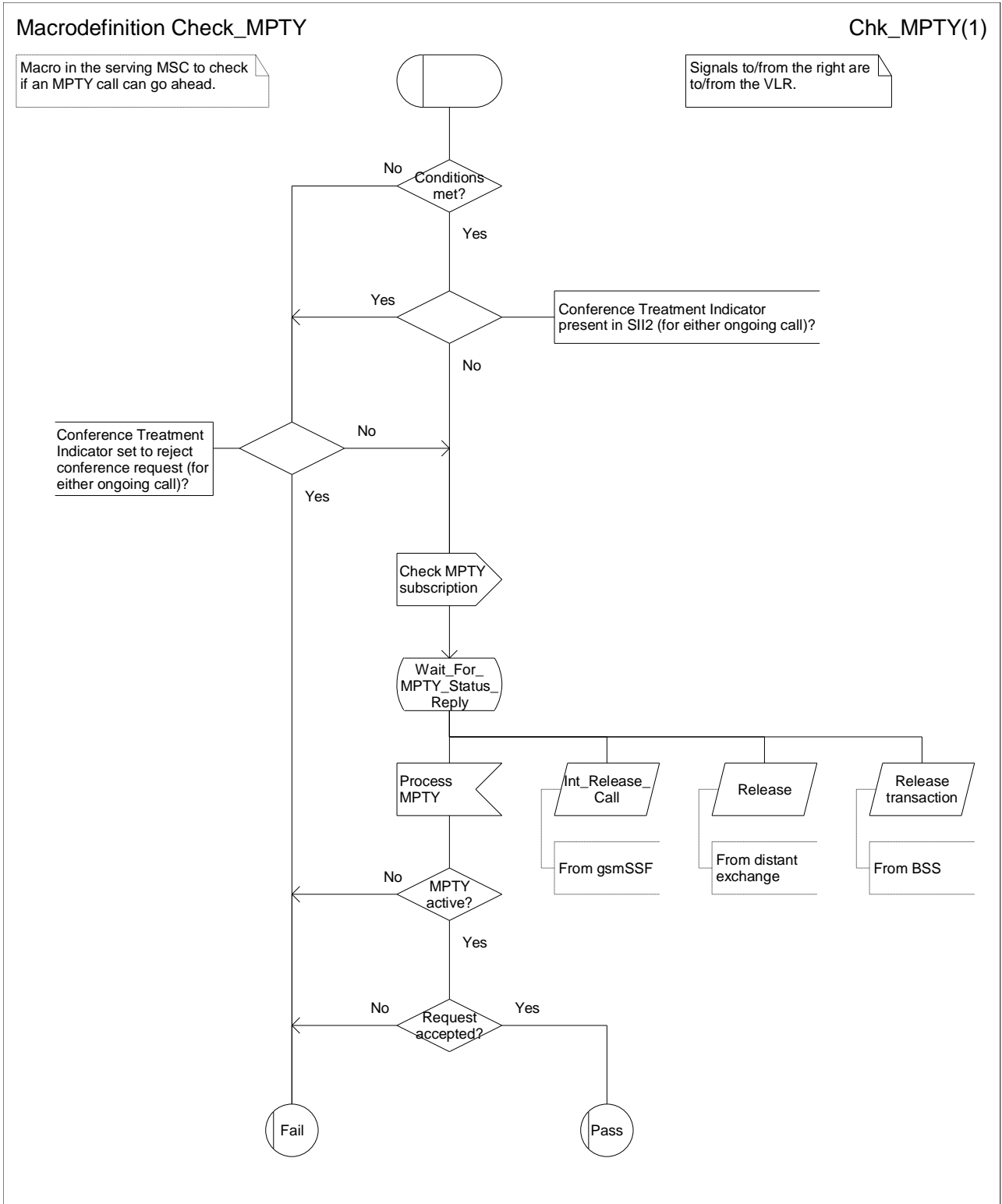
Figure 1.3: Macro Check_MPTY
