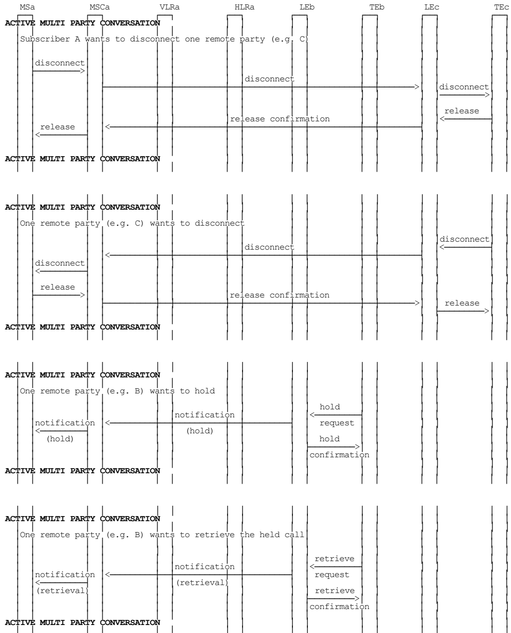
Figure 1.5 (sheet 2 of 7): Information flow for Multi Party service
