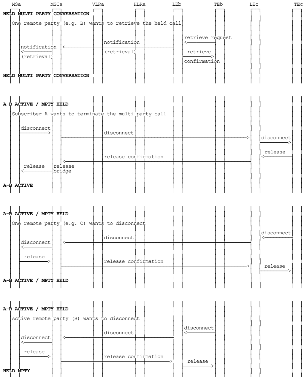
Figure 1.5 (sheet 5 of 7): Information flow for Multi Party service
