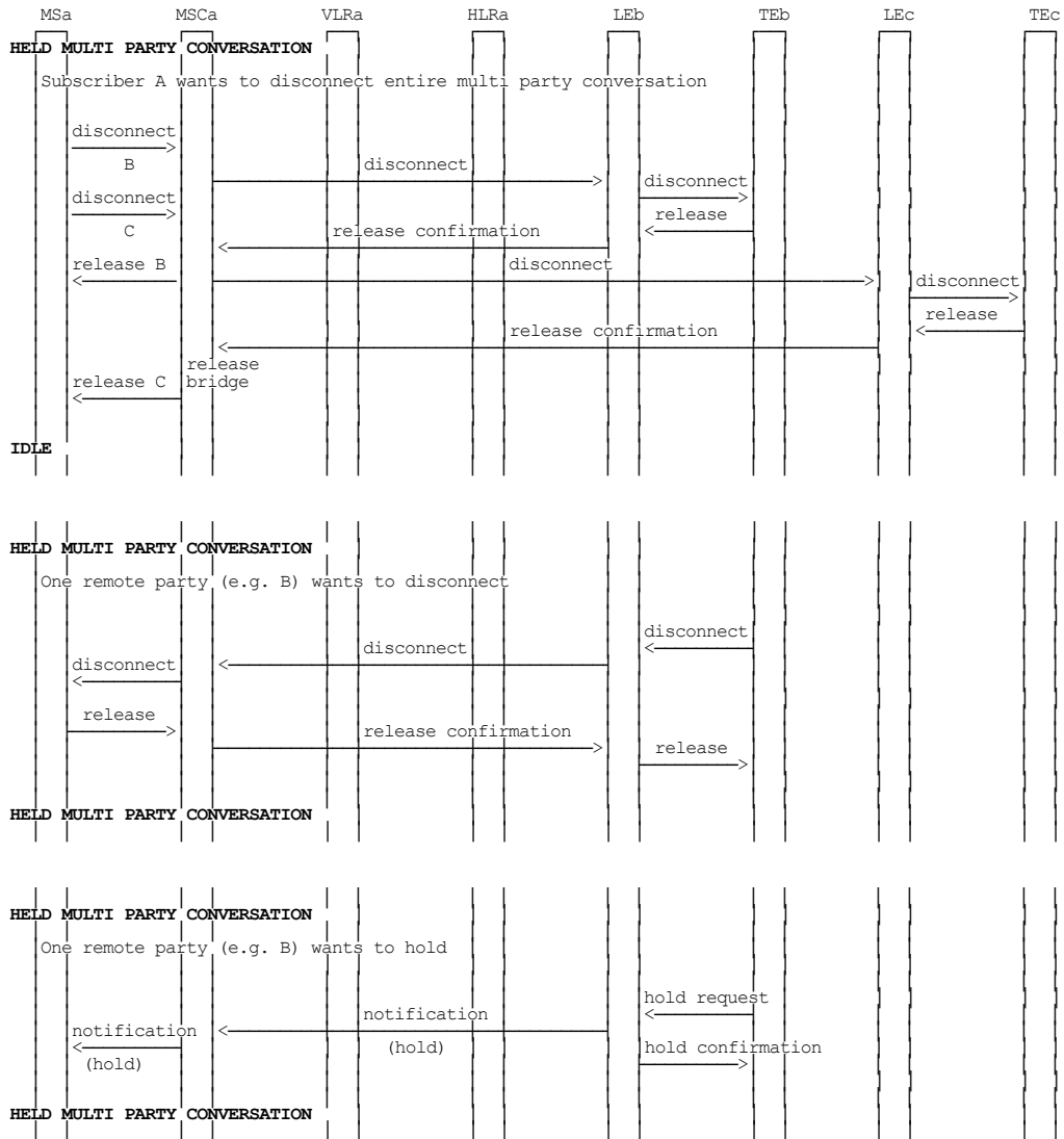
Figure 1.5 (sheet 4 of 7): Information flow for Multi Party service
