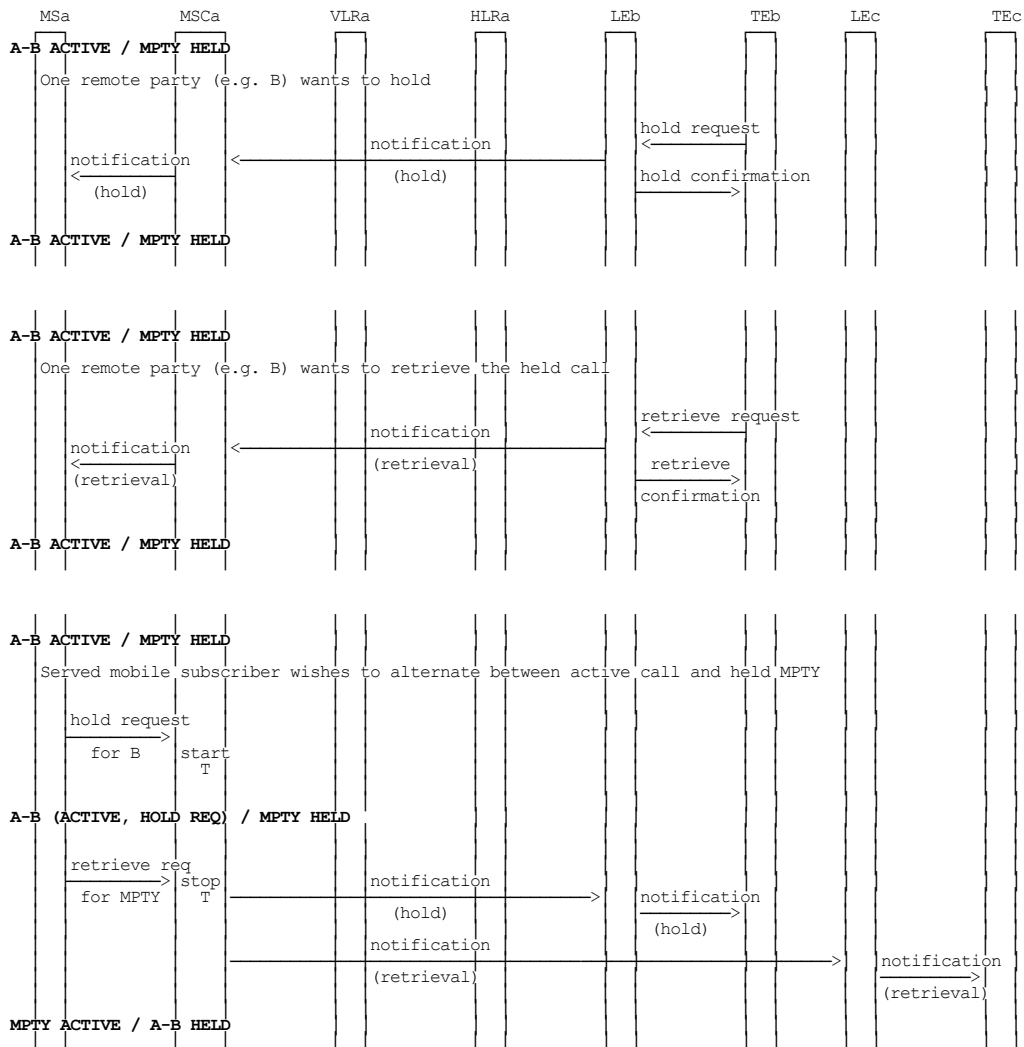
Figure 1.5 (sheet 7 of 7): Information flow for Multi Party service
