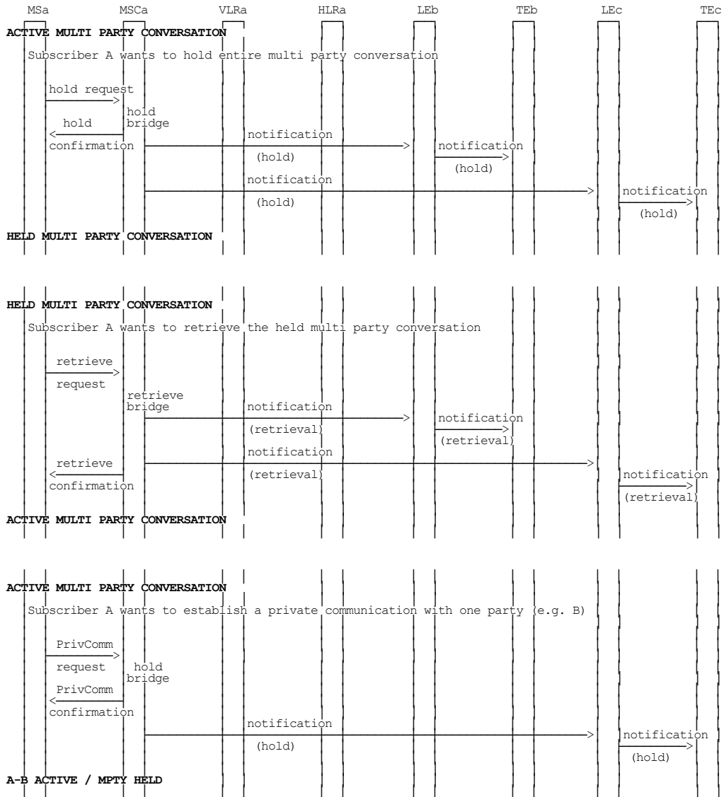
Figure 1.5 (sheet 3 of 7): Information flow for Multi Party service
