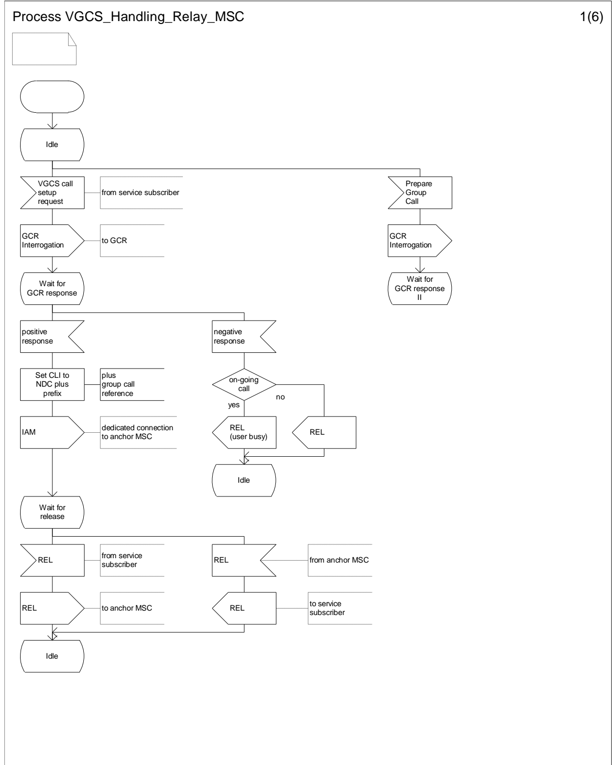
Figure 10: The VGCS handling process in the relay MSC (sheet 1 of 6)
