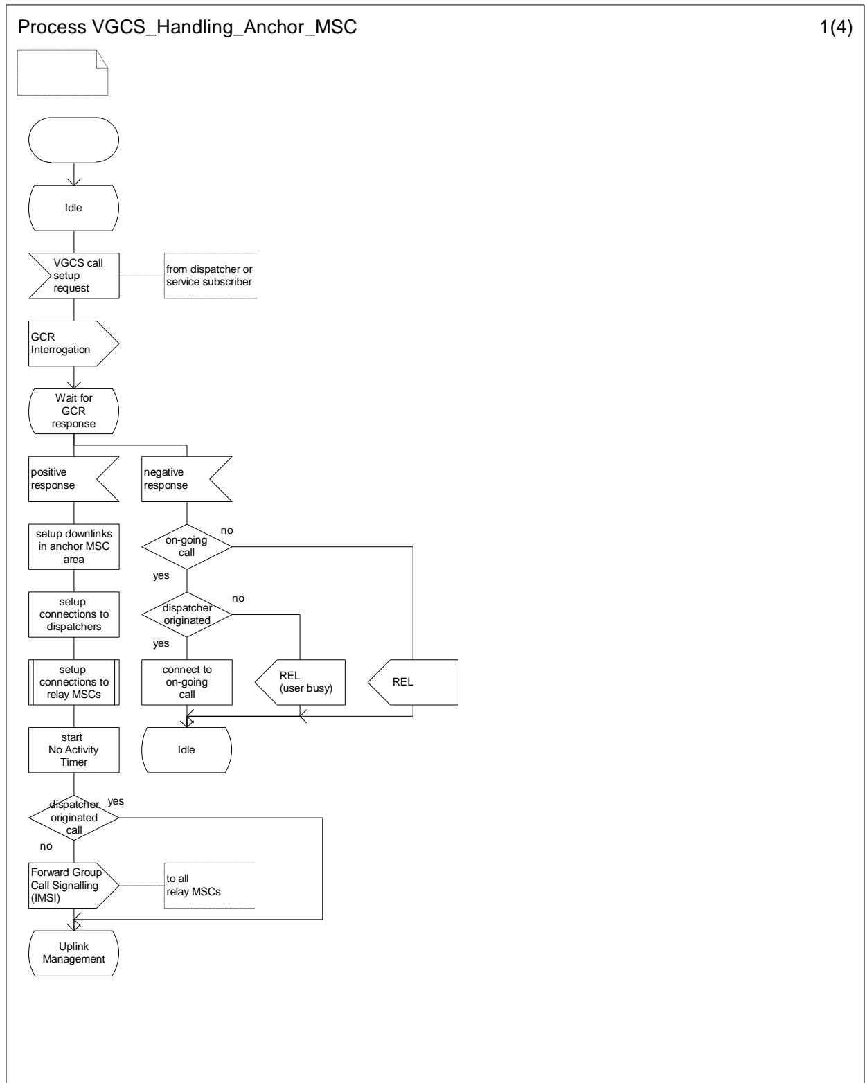
Figure 8: The VGCS handling process in the anchor MSC (sheet 1 of 4)
