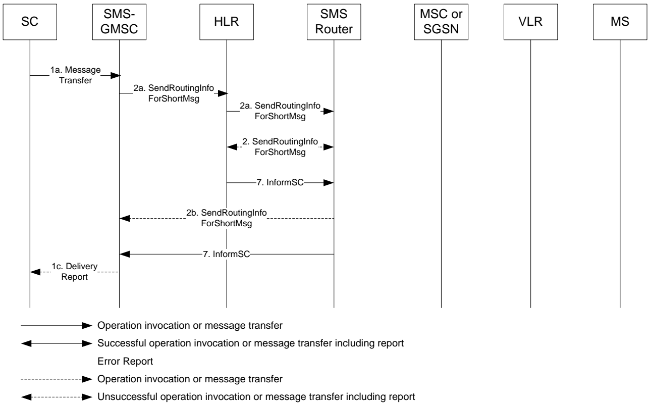
Figure 15ca) Short message transfer attempt via the SMS Router failing due to negative outcome of HLR information retrieval
