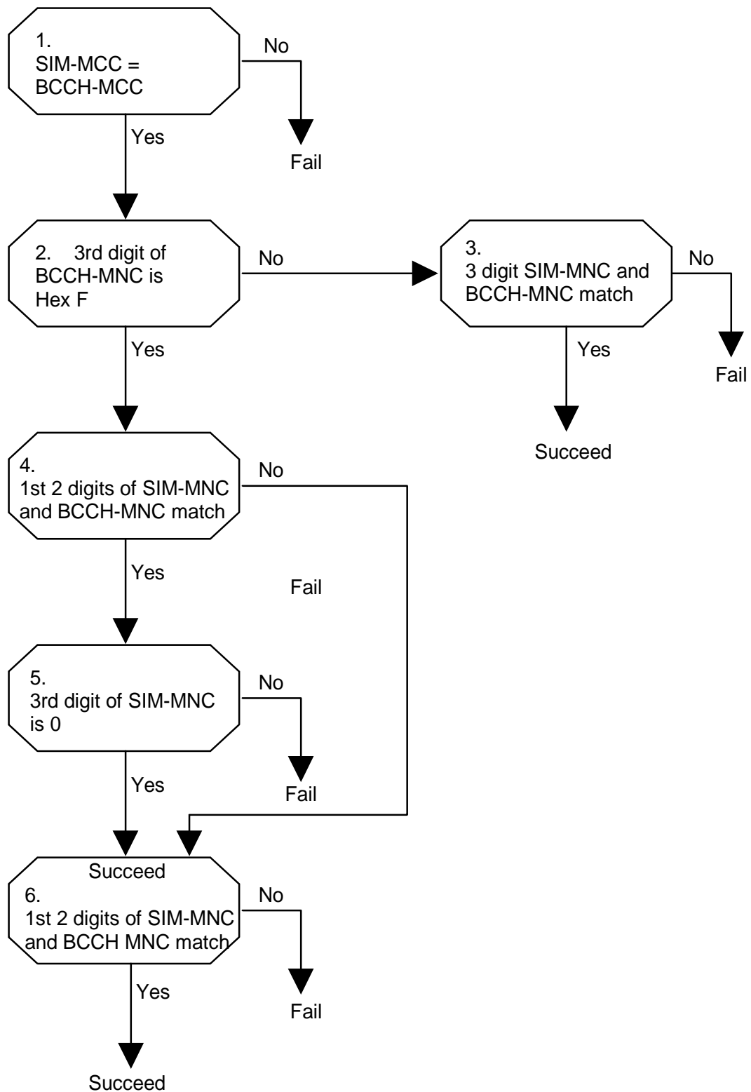
Figure A.2: HPLMN Matching Criteria Logic Flow for mobiles which support PCS1900 for NA
