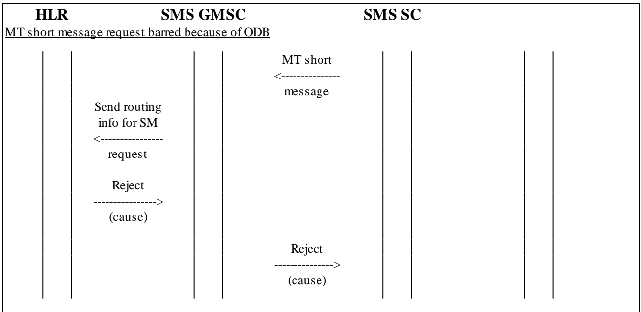
Figure 2.2.2/2: Operator Determined Barring of Mobile Terminated Short Messages
