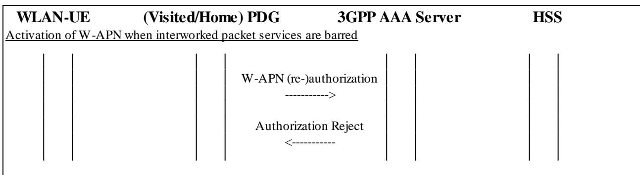
Figure 2.8.2/1: Authorization attempt of a interworked packet services when the WLAN-UE is connecting via a PDG located either in Visited or Home PLMN
