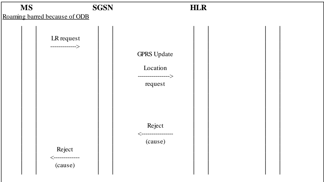
Figure 2.3.2/2: Operator Determined Barring of Roaming invocation in HLR. Roaming in a prohibited SGSN
