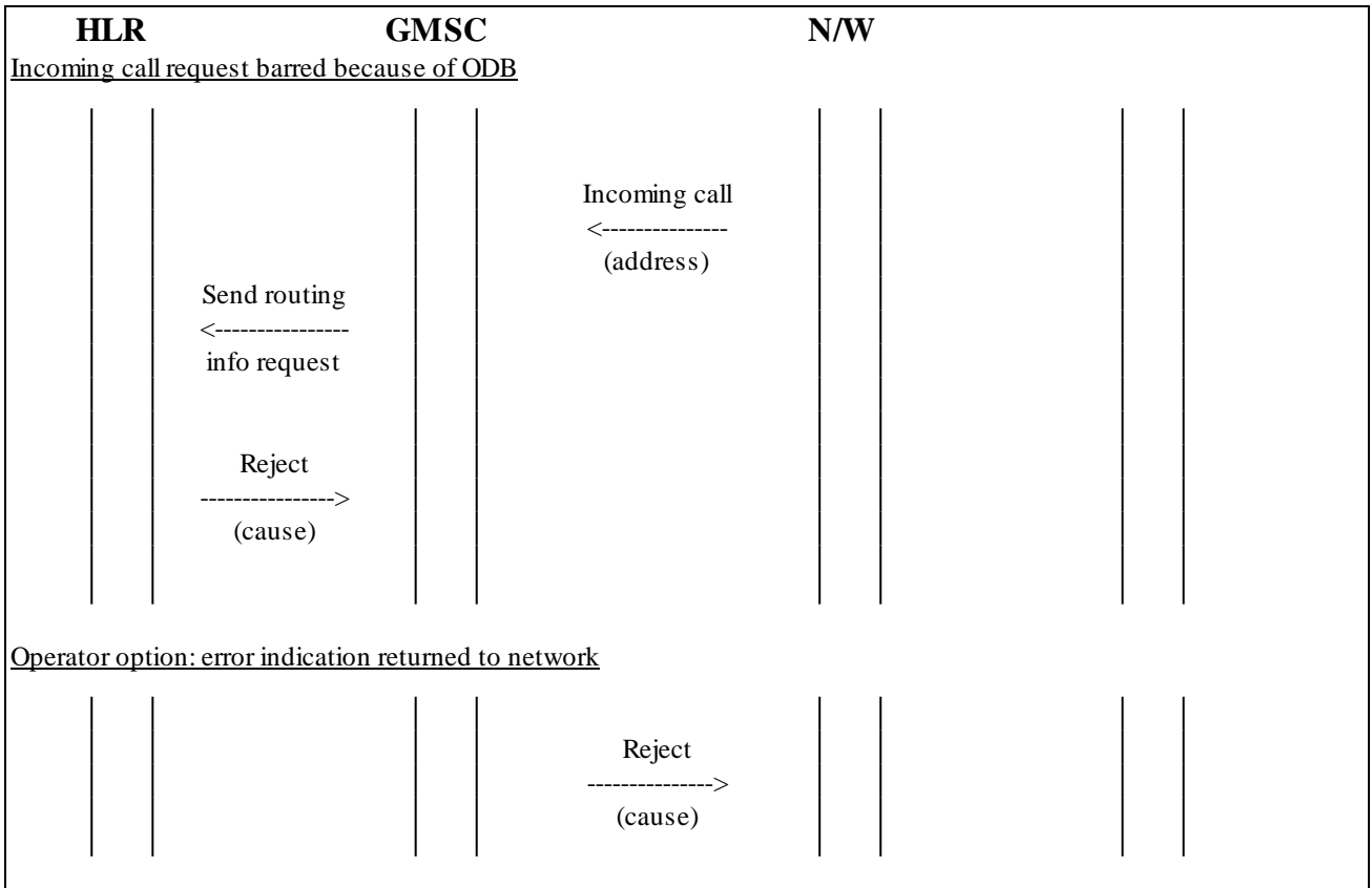
Figure 2.2.2/1: Operator Determined Barring of Incoming Calls
