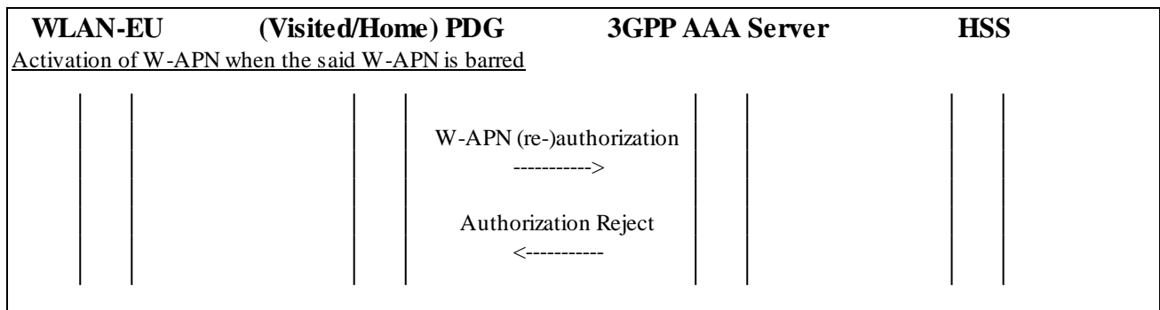
Figure 2.8.3/1: Authorization attempt of a W-APN when the WLAN-UE is connecting via a PDG located either in Visited or Home PLMN
