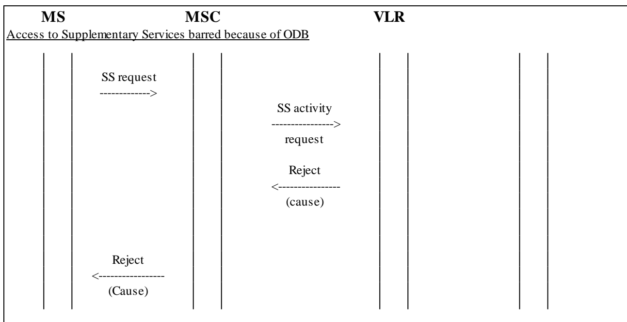
Figure 2.4.2/2: Operator Determined Barring of Access to Supplementary Services in the VLR
