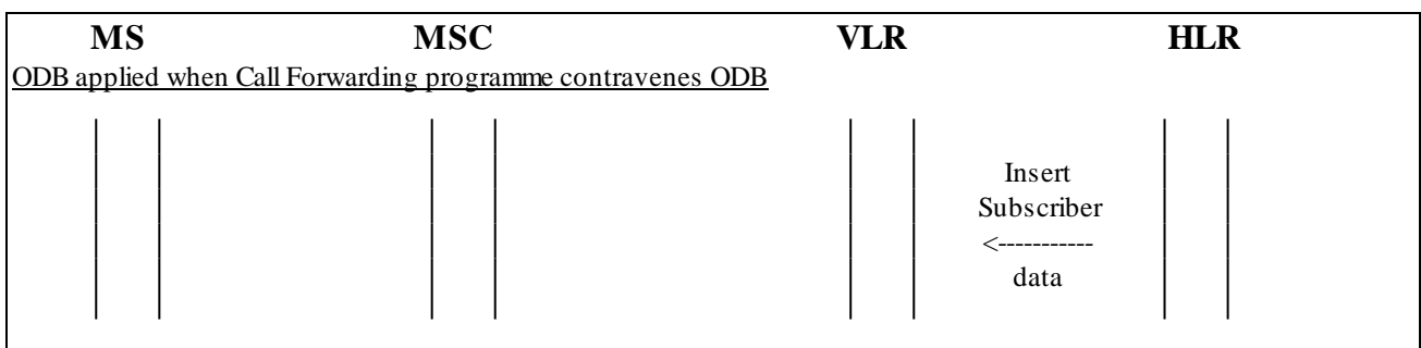
Figure 2.7.1/1: Effect of Operator Determined Barring on Call Forwarding programme
