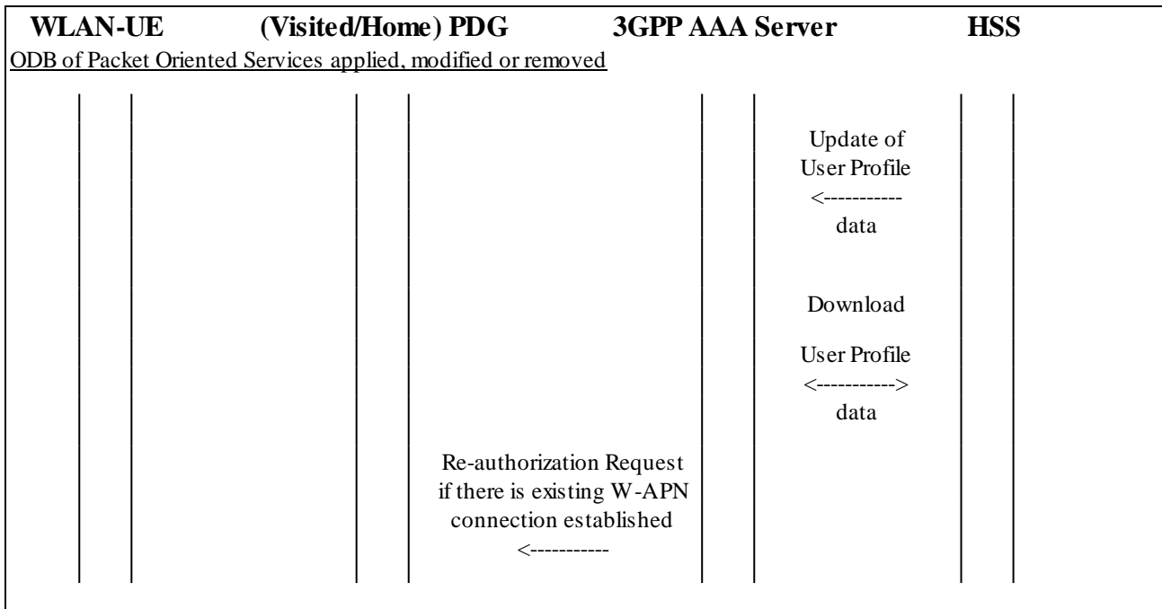
Figure 2.8.1/1: Transfer of updated User profile Data to 3GPP AAA Server
