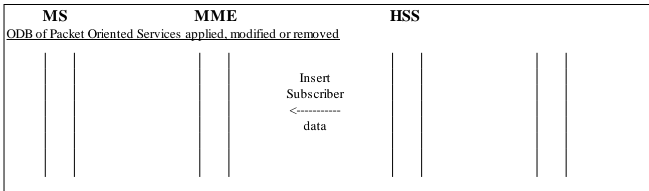
Figure 2.5A.1/1: Transfer of updated subscription information to MME
