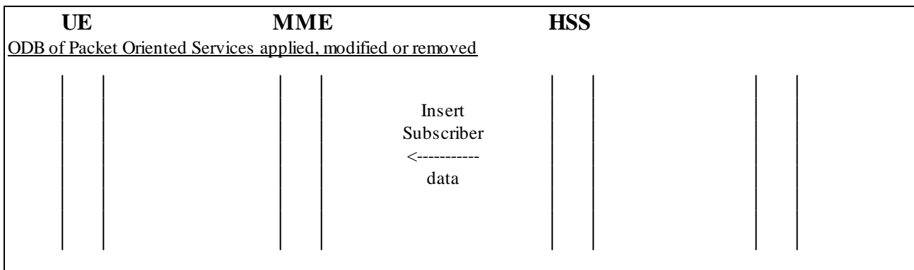
Figure 2.6B.1/1: Transfer of updated subscription information to MME
