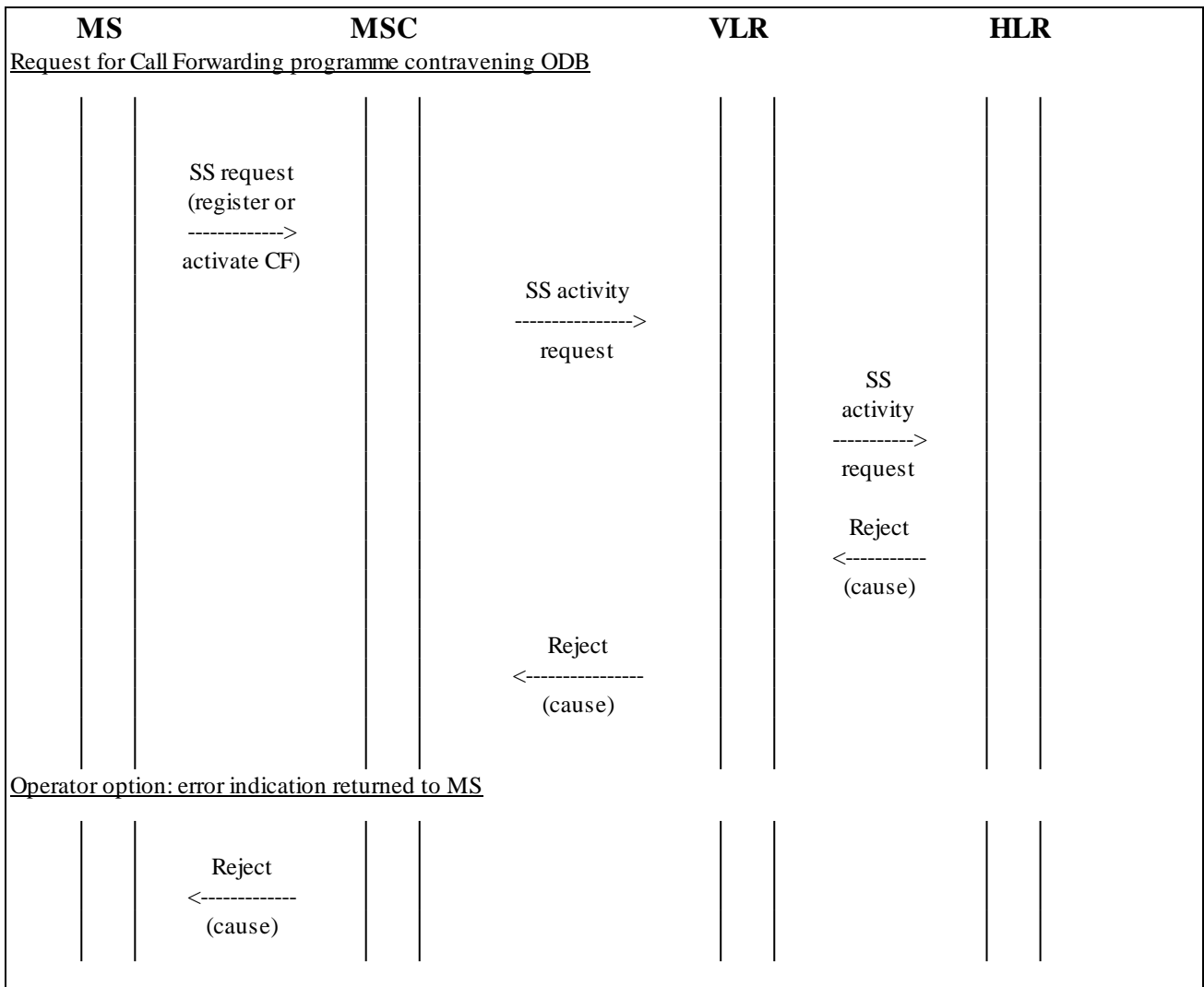
Figure 2.7.1/2: Interaction between Operator Determined Barring and Call Forwarding
