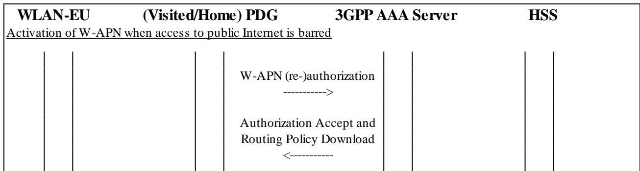
Figure 2.8.4/1: Authorization of a W-APN when public Internet access is barred
