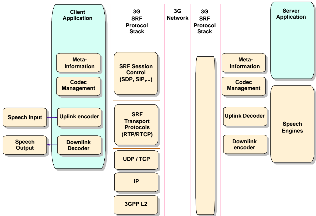
Figure 14 – Possible architecture for integrating SRF framework within 3GPP protocol stack and architecture.
