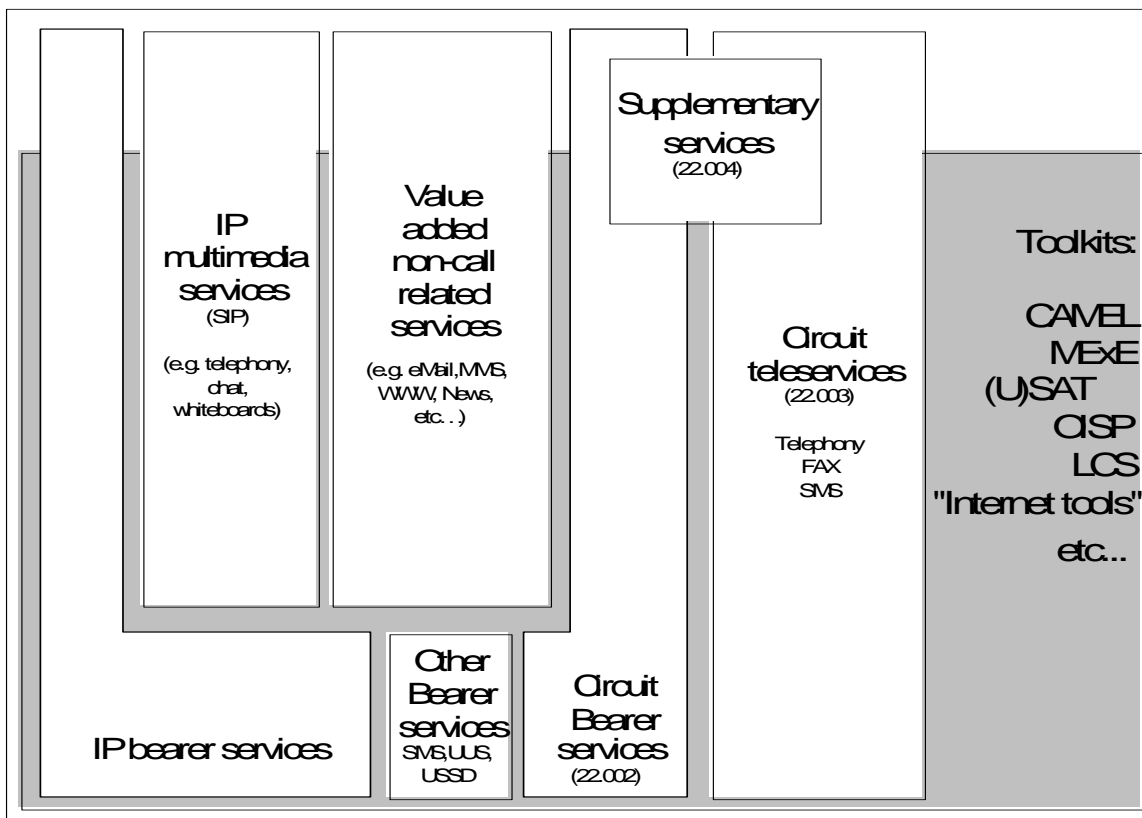
Figure 1: Service classification
