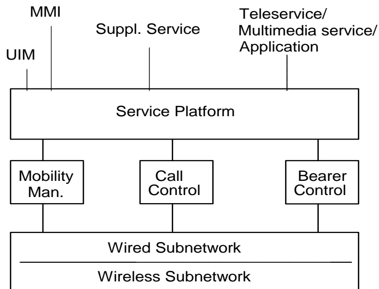
Figure 2: Service Architecture
