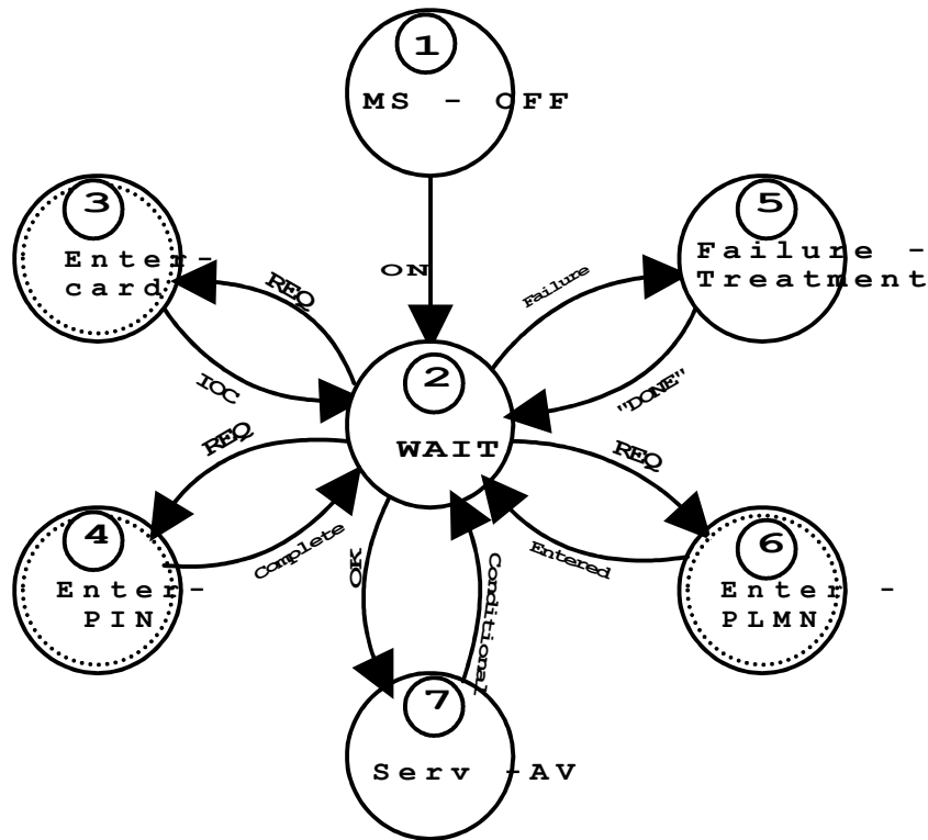
Figure A.1: Mealy-graph for the UE access procedure
