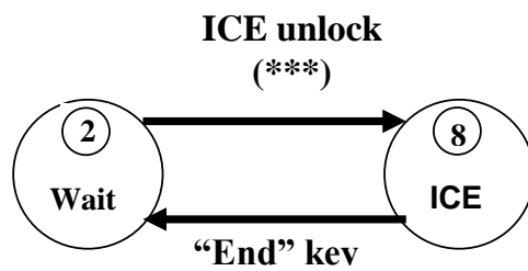
Figure A.2: Mealy-graph for the In Case of Emergency access procedure
