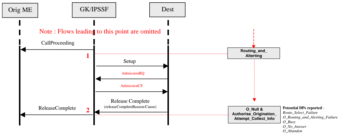
Figure 12: H.323 message flows and corresponding CAMEL O-BCSM for the unsuccessful establishment (other than admission refusal)
