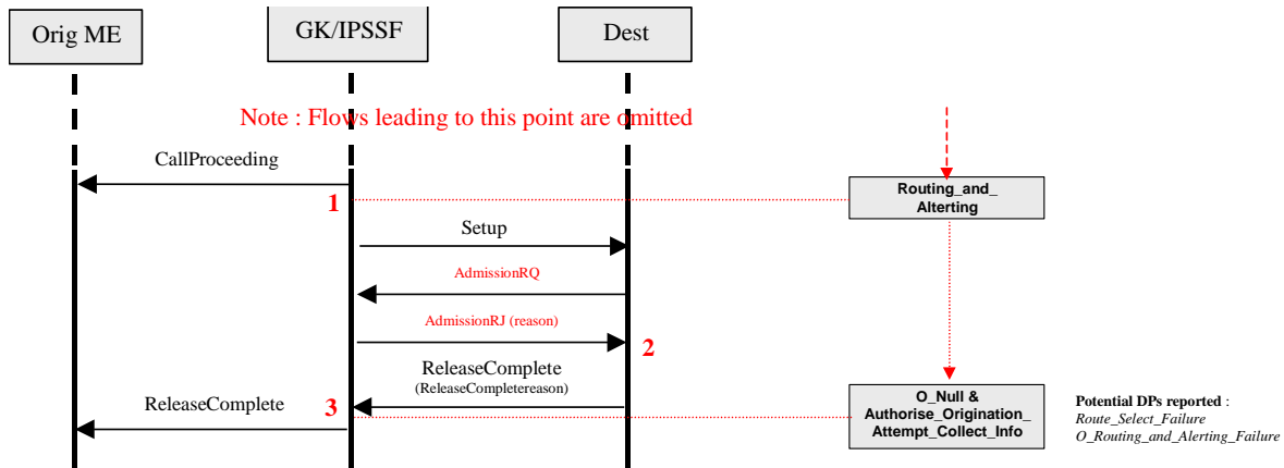
Figure 11: H.323 message flows and corresponding CAMEL O-BCSM for the case where the destination is refused permission to accept the call by the gatekeeper
