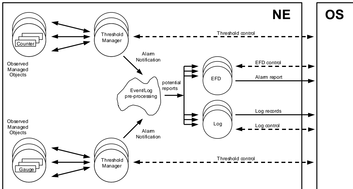
Figure 2: Inter-relationship of counters and gauges with thresholds
