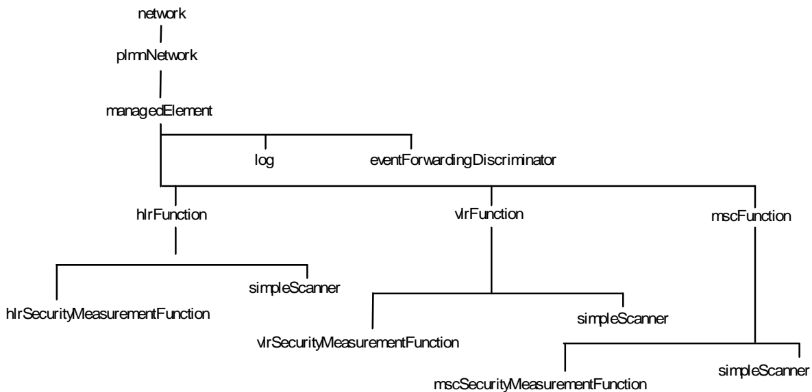
Figure C.1: GSM 12.03 Security Measurement Object Class Containment
