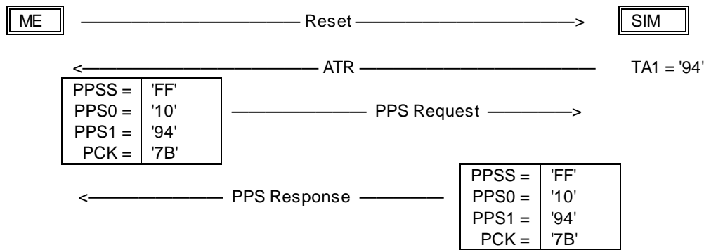
Figure 2: PPS procedure requesting enhanced speed values (F=512, D=8, see clause 5.8.3)
