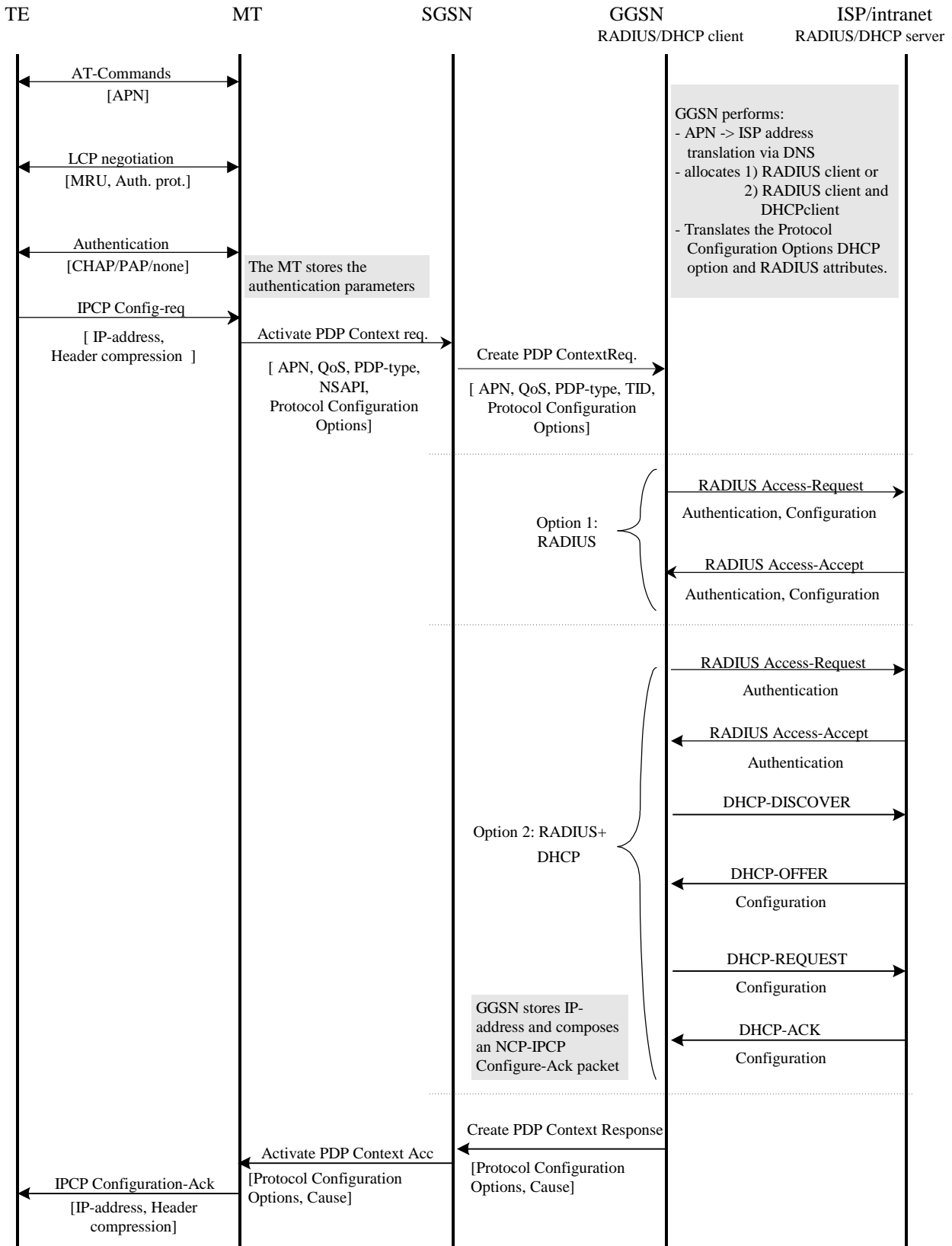
Figure 12: Example where PPP is used as layer 2 protocol over the R reference point
