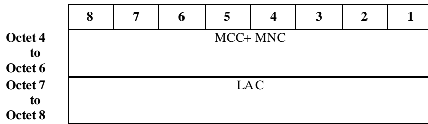
Figure 10.19.4/3GPP TS 09.31: Coding of Network Element Identification using the MCC + MNC + LAC
